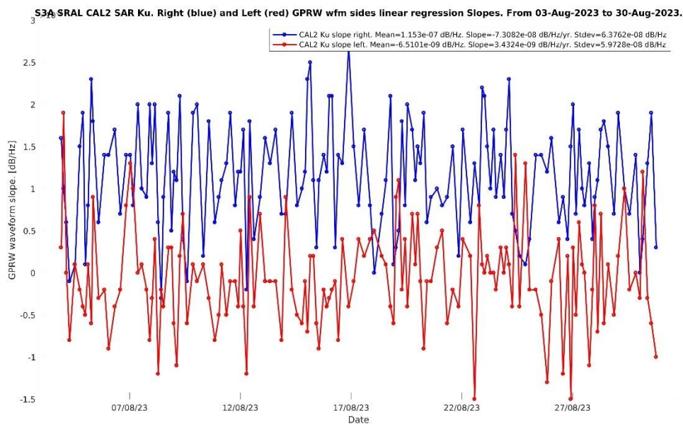
Figure 4-21. S3A CAL2 SAR Ku waveforms right (blue) and left (red) sides Slope over the period.
