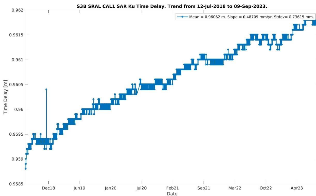
Figure 4-34. S3B CAL1 SAR Ku Time Delay Whole Mission Trend.
