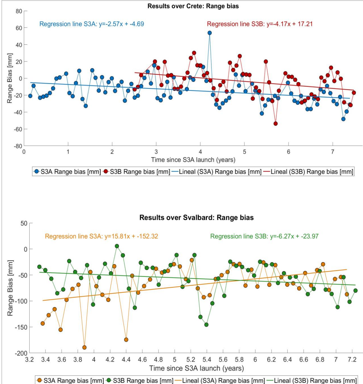
Figure 5-1. Range Bias Results.
