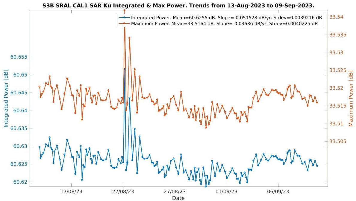
Figure 4-6. S3B CAL1 SAR Ku Power Trend.
