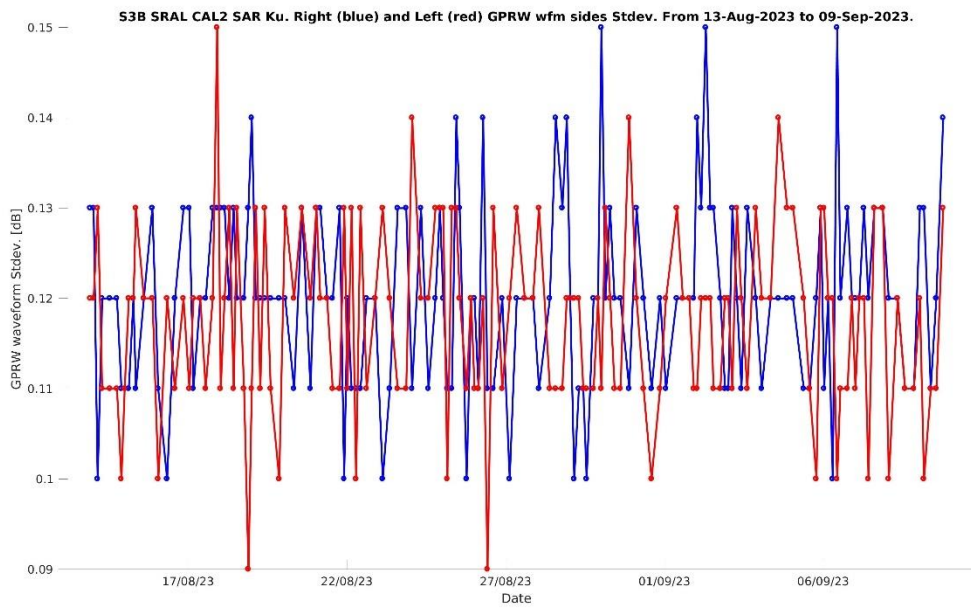
Figure 4-24. S3B CAL2 SAR Ku waveforms right (blue) and left (red) sides Standard Deviation over the period.
