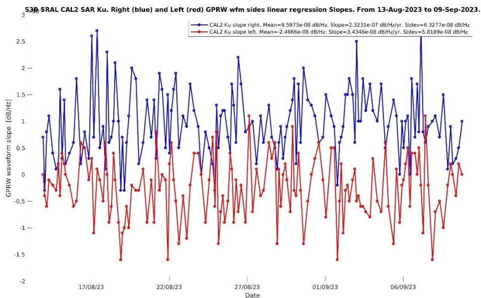
Figure 4-22. S3B CAL2 SAR Ku waveforms right (blue) and left (red) sides Slope over the period.
