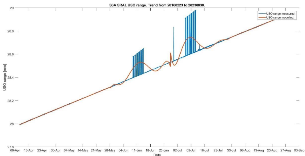
Figure 2-1. S3A range anomaly
