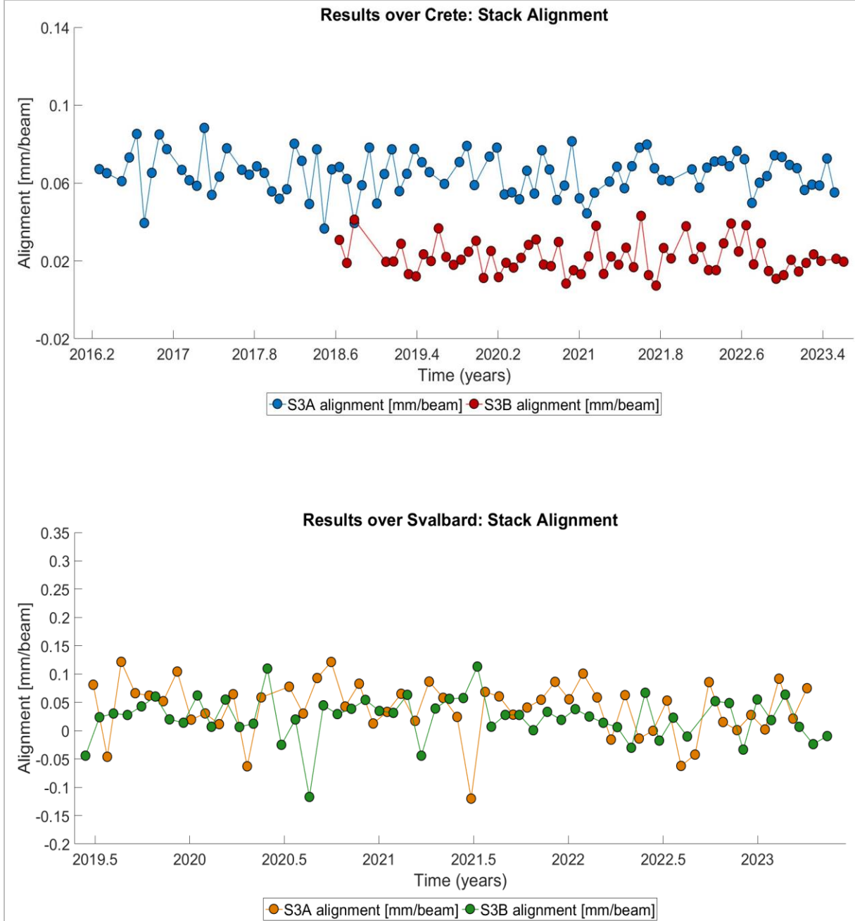
Figure 5-3. Alignment Results.
