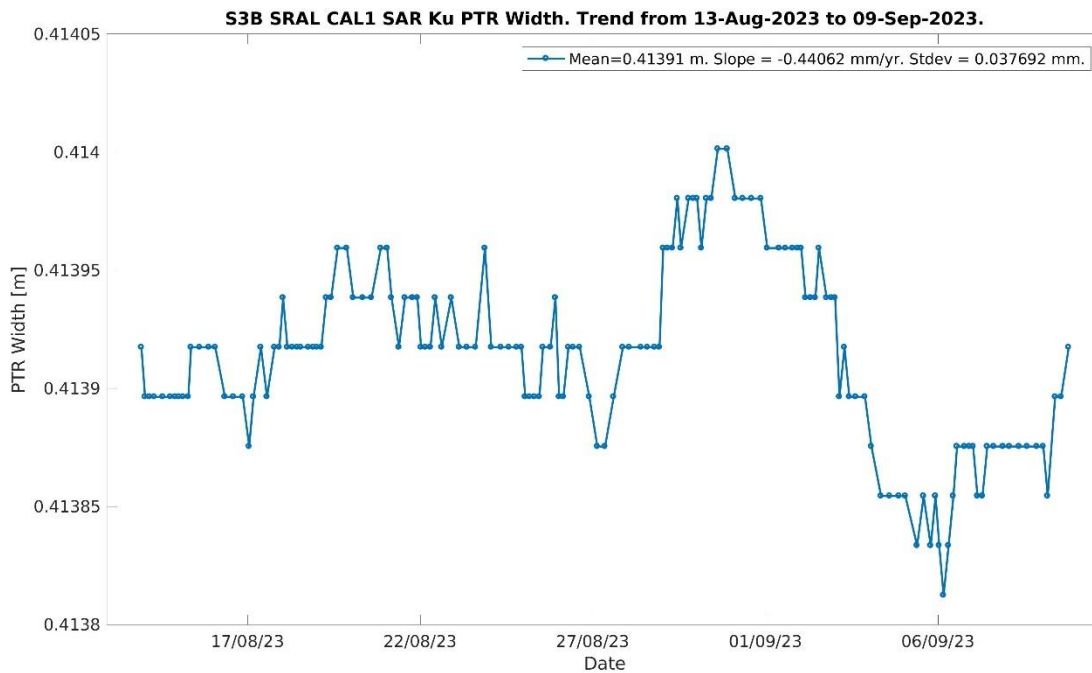
Figure 4-8. S3B CAL1 SAR Ku PTR width trend.
