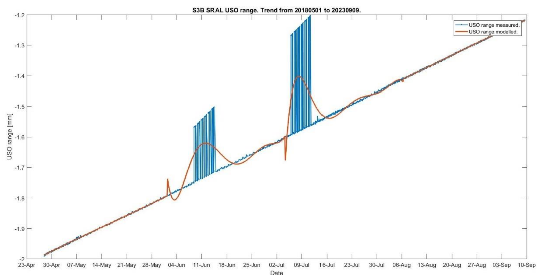
Figure 2-2. S3B range anomaly
