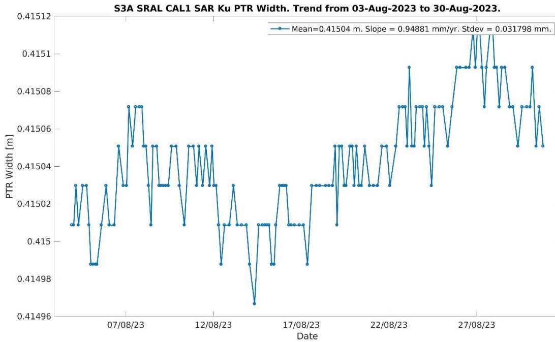
Figure 4-7. S3A CAL1 SAR Ku PTR width trend.
