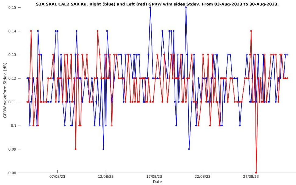
Figure 4-23. S3A CAL2 SAR Ku waveforms right (blue) and left (red) sides Standard Deviation over the period.
