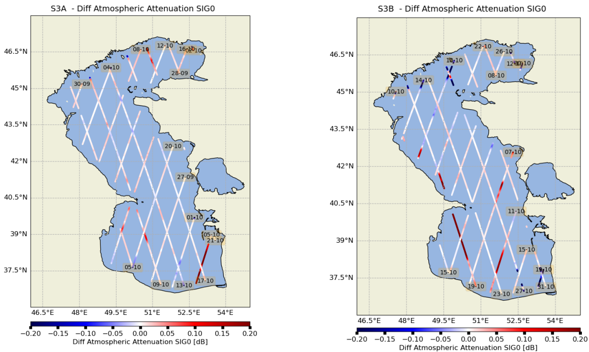
Figure 27: Difference MWR-ECMWF of Atmospheric attenuation of Sigma0 (SAR) on Caspian Sea for Sentinel-3A and Sentinel-3B
