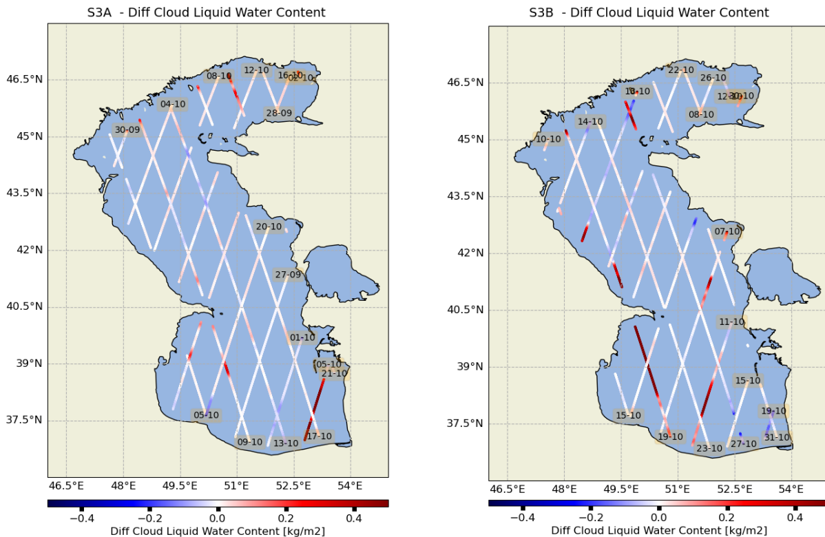
Figure 31: Difference MWR-ECMWF of Cloud liquid water content on Caspian Sea for Sentinel-3A and Sentinel-3B
