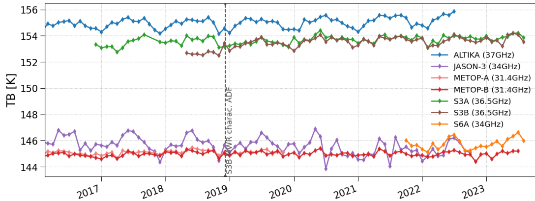
Figure 18 : Coldest temperature over ocean for the liquid water channel S3AB, SARAL/AltiKa, Jason2, Jason3 and Metop-A/AMSU-A
