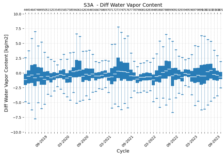
Figure 29: Difference MWR-ECMWF of Water vapor on Caspian Sea for Sentinel-3A and Sentinel-3B
