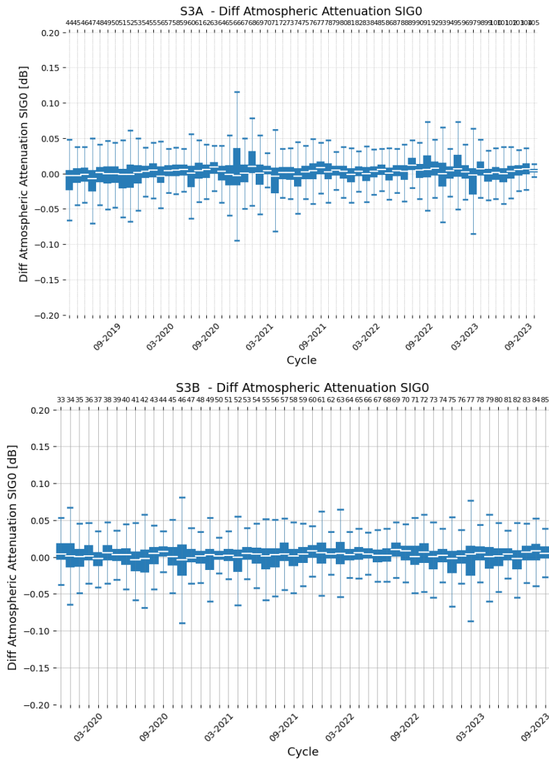
Figure 28: Timeseries of difference MWR-ECMWF of Atmospheric attenuation of Sigma0 (SAR) for Sentinel-3A (top) and Sentinel-3B (bottom)
