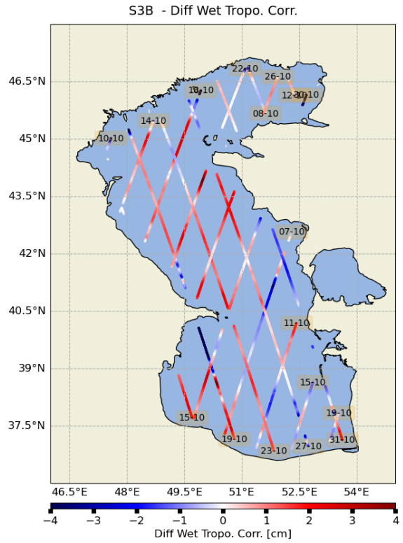
Figure 25: Difference MWR-ECMWF of WTC (SAR) on Caspian Sea for Sentinel-3A and Sentinel-3B
