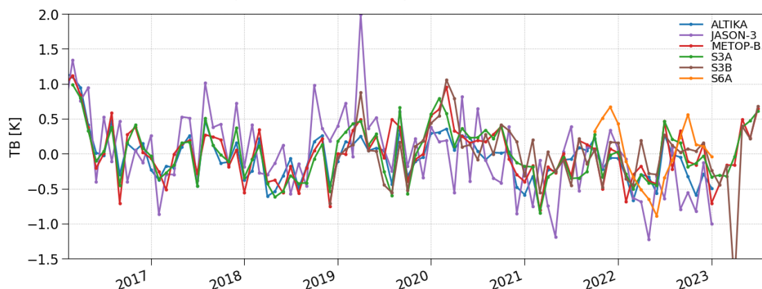
Deseasoned mean of Brightness Temperature (23.8GHz channel) over Amazon forest
