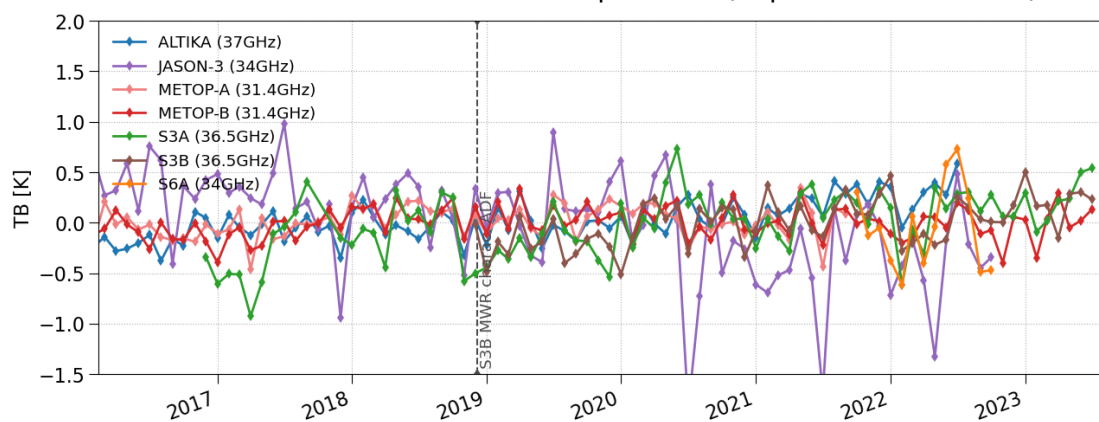
Residuals of ocean coldest Temperature (Liquid Water channel)
