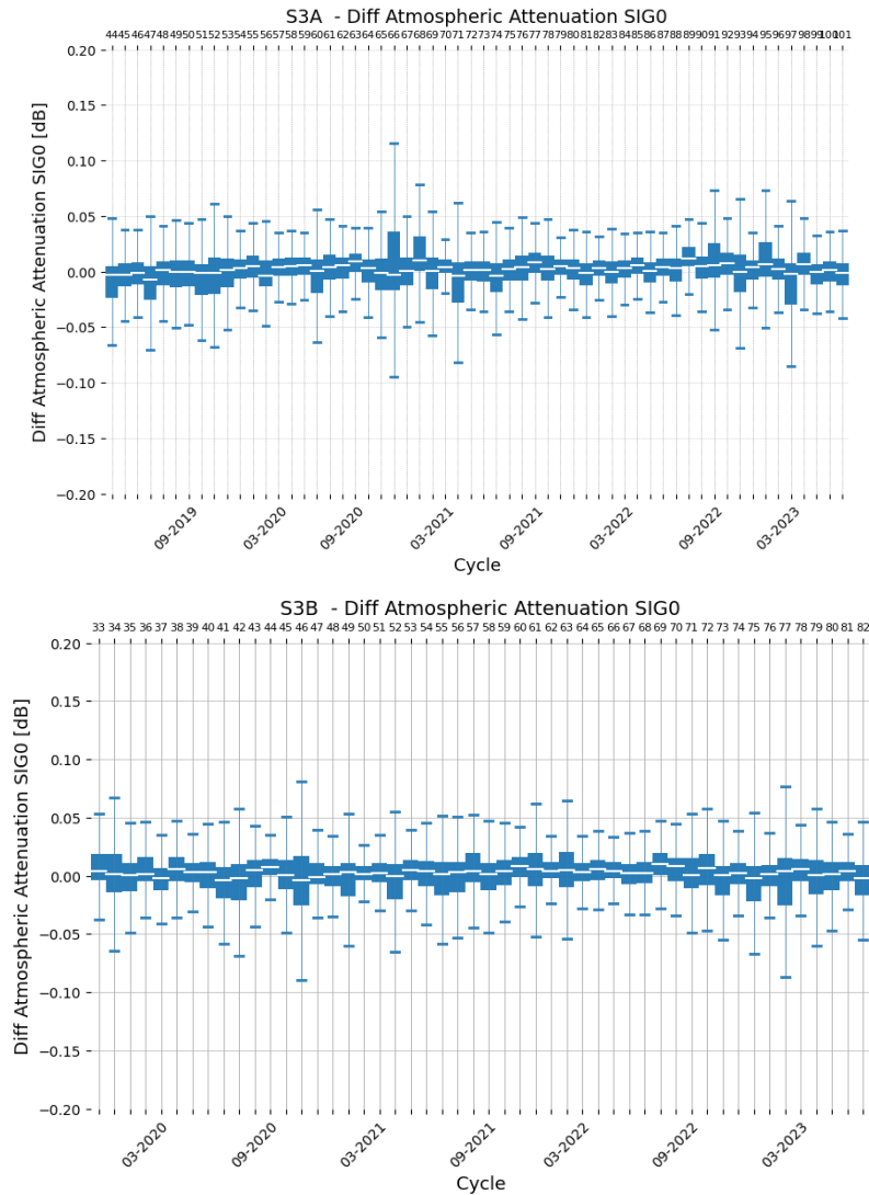
Figure 27: Difference MWR-ECMWF of Atmospheric attenuation of Sigma0 (SAR) on Caspian Sea for Sentinel-3A and Sentinel-3B
