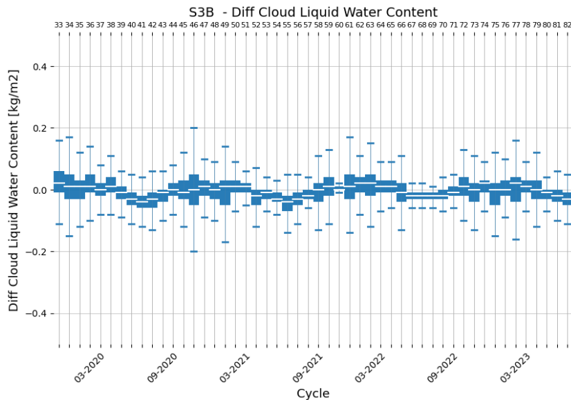
Figure 32: Timeseries of difference MWR-ECMWF of Cloud liquid water content for Sentinel-3A (top) and Sentinel-3B (bottom)
