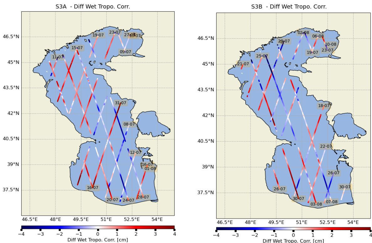
Figure 25: Difference MWR-ECMWF of WTC (SAR) on Caspian Sea for Sentinel-3A and Sentinel-3B
