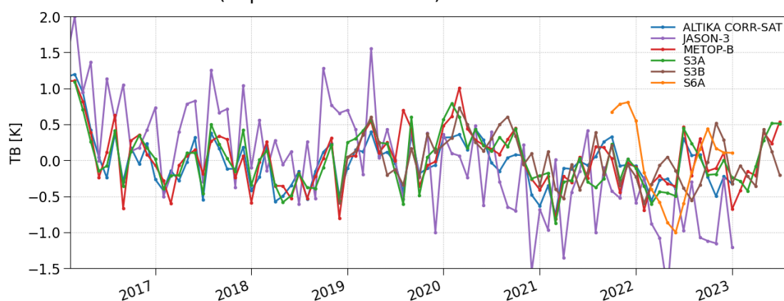
Deseasoned mean of Brightness Temperature (Liquid Water channel) over Amazon forest
