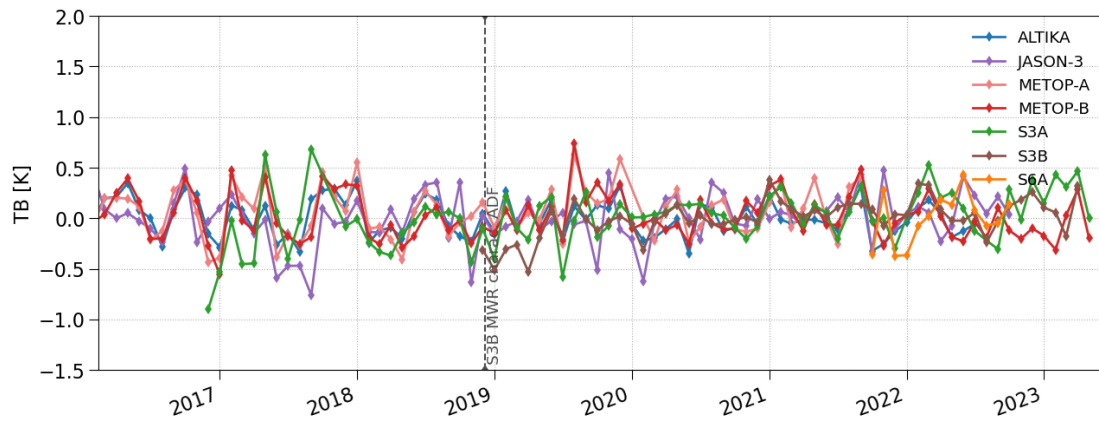
Residuals of ocean coldest Temperature (23.8Ghz channel)
