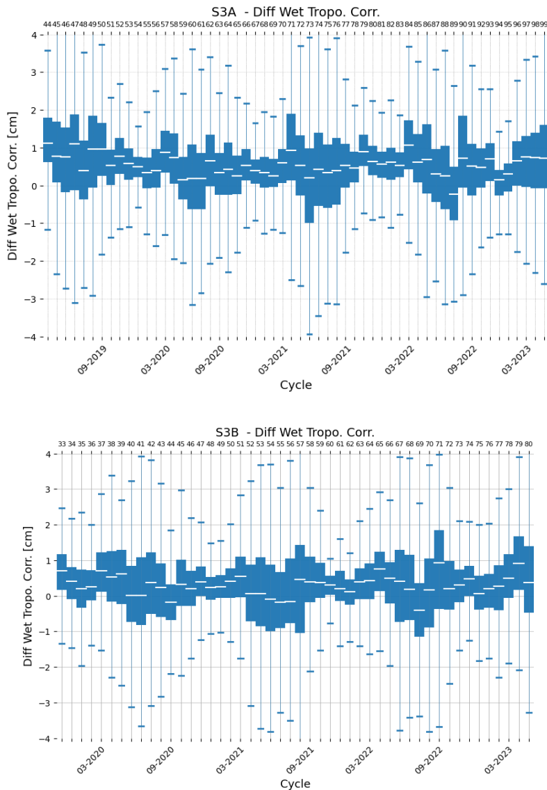
Figure 26: Timeseries of difference MWR-ECMWF of WTC (SAR) for Sentinel-3A (top) and Sentinel-3B (bottom)
