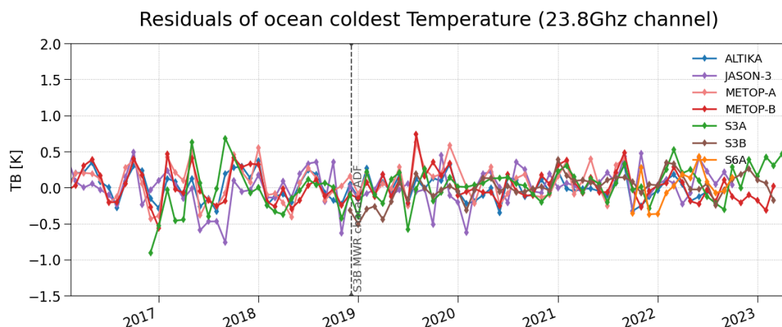
Figure 19 : Residuals after removal of yearly signal over ocean at 23.8GHz for S3A/B, SARAL/AltiKa, Jason3, S6A, and Metop-A/AMSU-A
