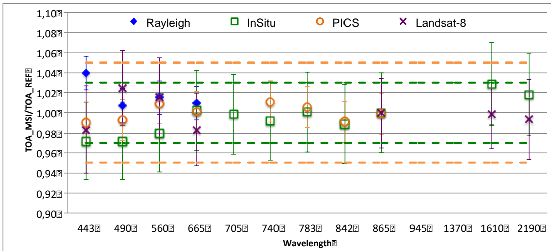
Figure 3: Comparison of radiometric accuracy for all spectral bands (except B10 and B9): ratio of S2A measurement on reference. Error bars indicate the method uncertainty.
