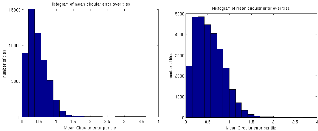
Figure 2: Histogram of the multi-temporal performance for S2A (left) and S2B (right, different scale). The current performance is 10 m (S2A) and 12 m (S2B), mean shift at 95% confidence.
