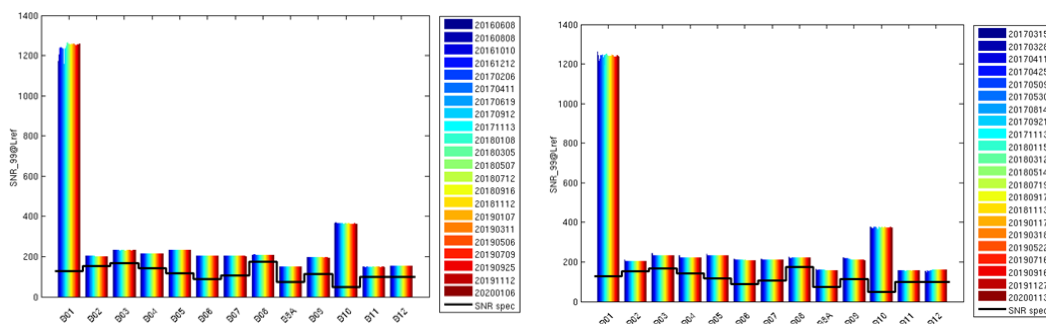
Figure 5: Evolution of the SNR performance for S2A since 08/06/2016 (left) and S2B since 15/03/2017 (right)
