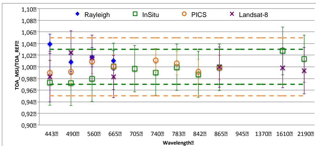
Figure 3: Comparison of radiometric accuracy for all spectral bands (except B10 and B09): ratio of S2A measurement on reference. Error bars indicate the method uncertainty.
