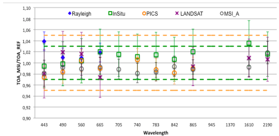
Figure 4: Comparison of radiometric accuracy for all spectral bands (except B09 & B10): ratio of S2B measurement on reference. Error bars indicate the method uncertainty.
