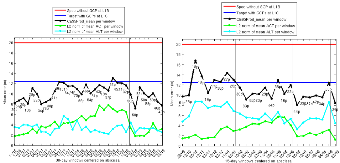
Figure 1: Geolocation performance for S2A (left) and S2B (right). The performance is computed over a sliding window of 30 days (S2A) and 15 days (S2B). Number of products used in the sliding window indicated for each point. (ACT= across track, ALT= along track). A vertical line indicates a geometric calibration event.
