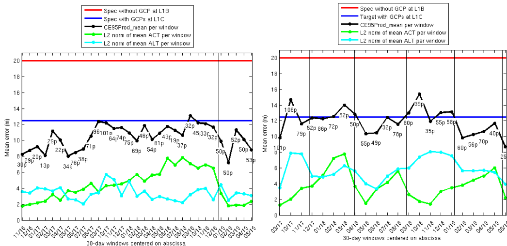
Figure 1: Geolocation performance for S2A (left) and S2B (right). The performance is computed over a sliding window of 30 days. Number of products used in the sliding window indicated for each point. (ACT= across track, ALT= along track). A vertical line indicates a geometric calibration event.
