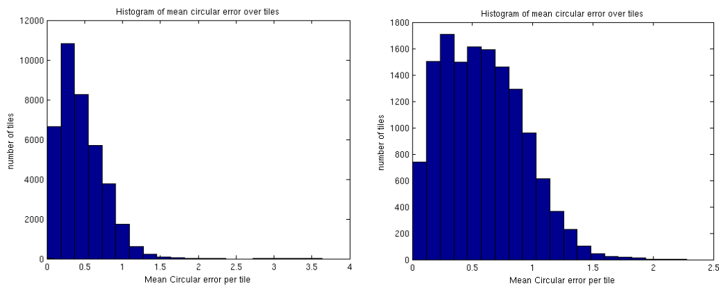
Figure 2: Histogram of the multi-temporal performance for S2A (left) and S2B (right, different scale). The current performance is 10 m (S2A) and 12 m (S2B) at 95% confidence.
