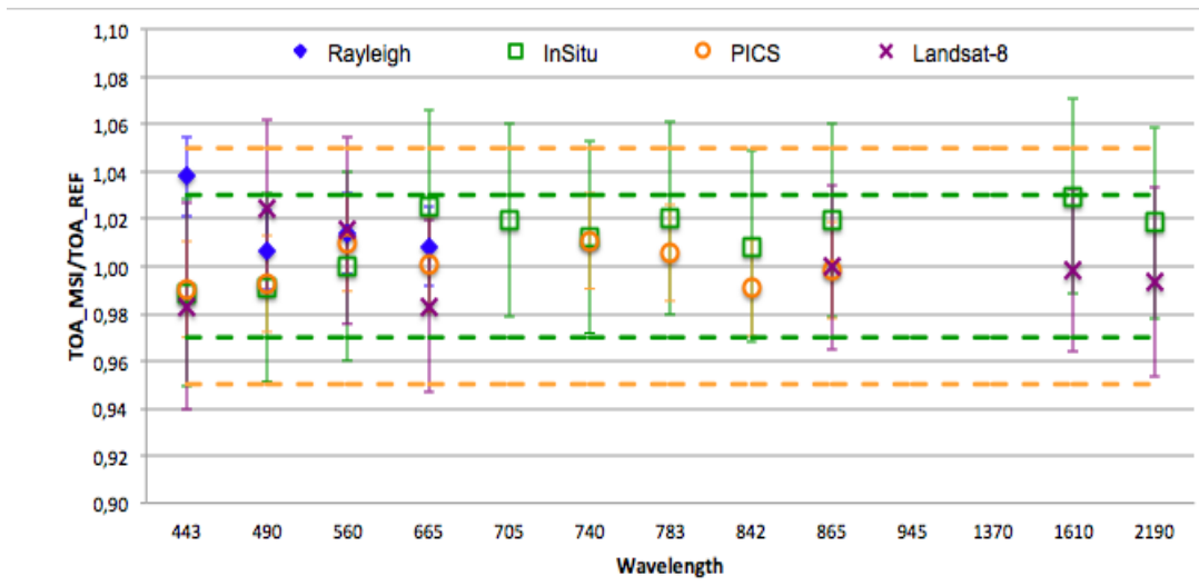
Figure 3: Comparison of radiometric accuracy for all spectral bands (except B10 and B9): ratio of S2A measurement on reference. Error bars indicate the method uncertainty.
