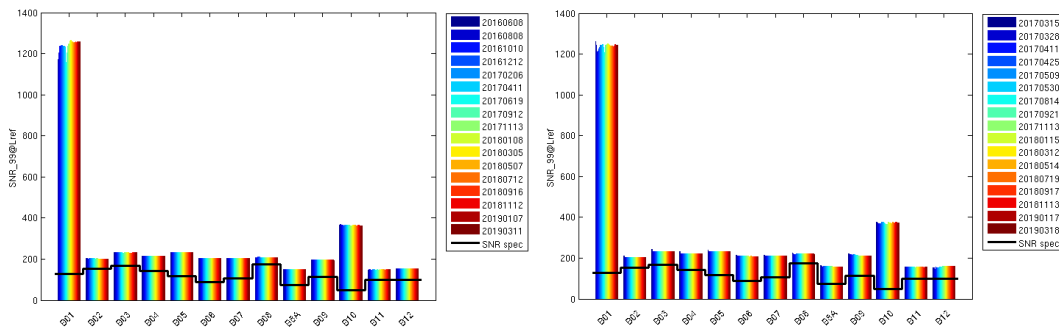
Figure 5: Evolution of the SNR performance or S2A since 08/06/2016 (left) and S2B since 15/03/2017 (right)
