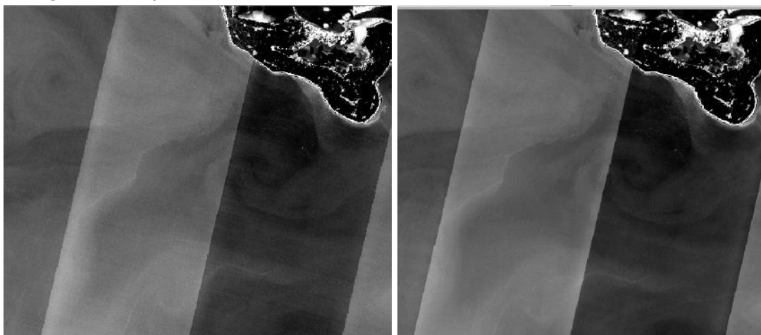
Figure 9: B01 image over sea with the current processing baseline 02.06 (Left) and the new processing baseline 02.07 (Right). Across-track lines due to correlated dark signal noise have been filtered.
