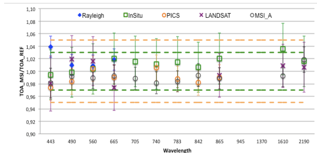
Figure 4: Comparison of radiometric accuracy for all spectral bands (except B09 & B10): ratio of S2B measurement on reference. Error bars indicate the method uncertainty.
