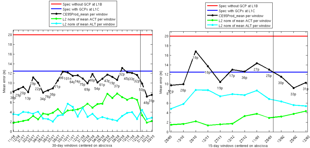
Figure 1: Geolocation performance for S2A (left) and S2B (right). The performance is computed over a sliding window of 30 days (S2A, left) or 15 days (S2B, right). Number of products used in the sliding window indicated for each point. (ACT= across track, ALT= along track). A vertical line indicates a geometric calibration event.
