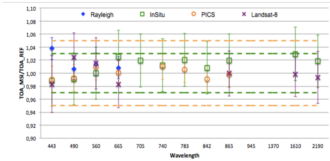
Figure 3: Comparison of radiometric accuracy for all spectral bands (except B10 and B09): ratio of S2A measurement on reference. Error bars indicate the method uncertainty.
