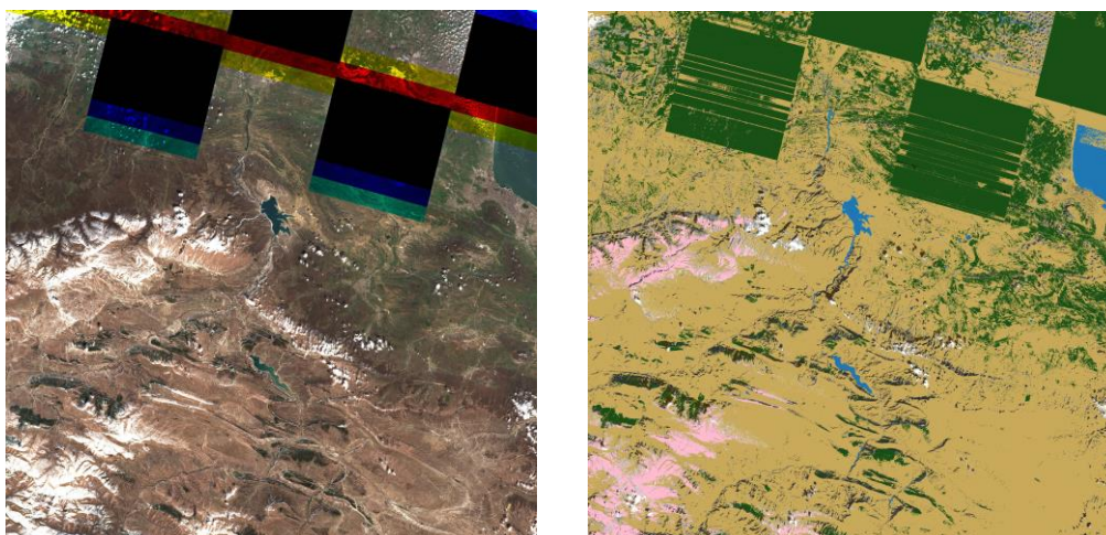
Figure 5-5: Left: TCI image of a product affected by missing packets. Right: Scene Classification Layer.
