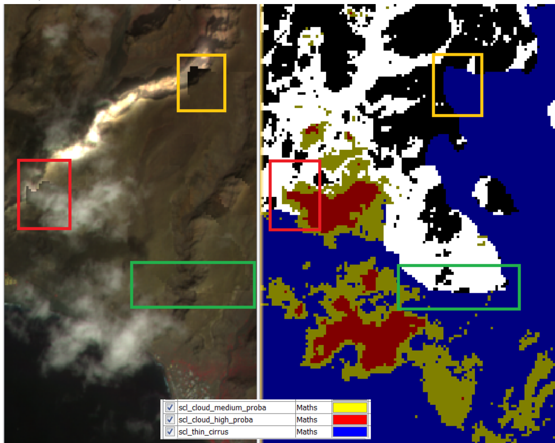
Figure 5-1: Visual artefacts at the edges of semi-transparent clouds.
