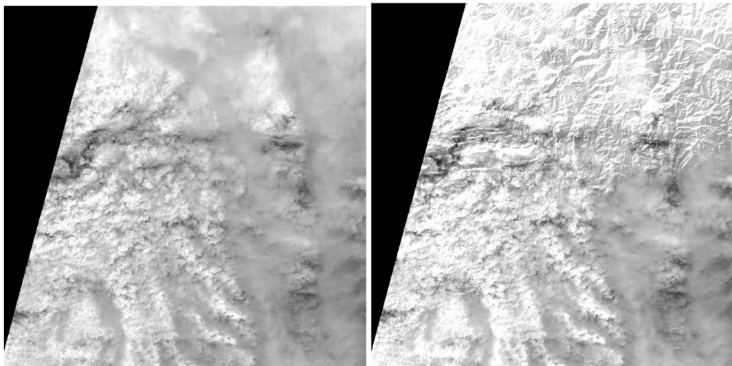
Figure 4-2: Band B04, Tile 32TLP from orbit S2B 7098. Left: L1C image; Right: L2A image. The topography seems to be visible through the opaque clouds. (Anomaly #4)
