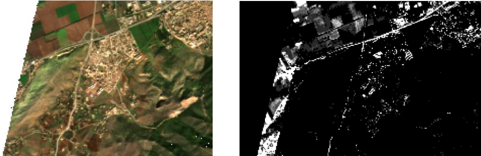
Figure 4-3: incorrect values of the cloud probability mask (CLDPRB) near the boundary of the swath. Left: L2A true colour image, Right: CLDPRB mask.
