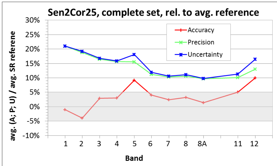
Figure 2-2: Average accuracy, precision and uncertainty relative to average surface reflectance reference per band for Sen2Cor version 2.5 based on the ACIX-dataset.
