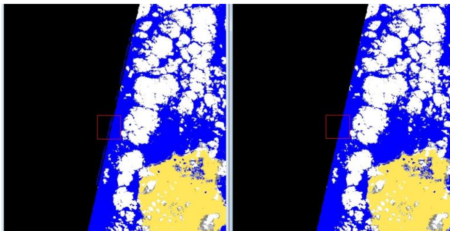
Figure 4-1: Incorrect No Data Mask (anomaly #2). Left: pixels incorrectly flagged as water (blue) near the swath edge. Right: same image after correction.
