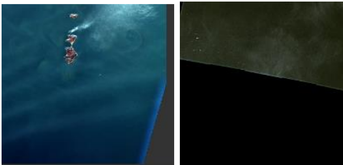
Figure 4-6: Halo near a swath edge (left) or data-strip end (right). Anomaly #66
