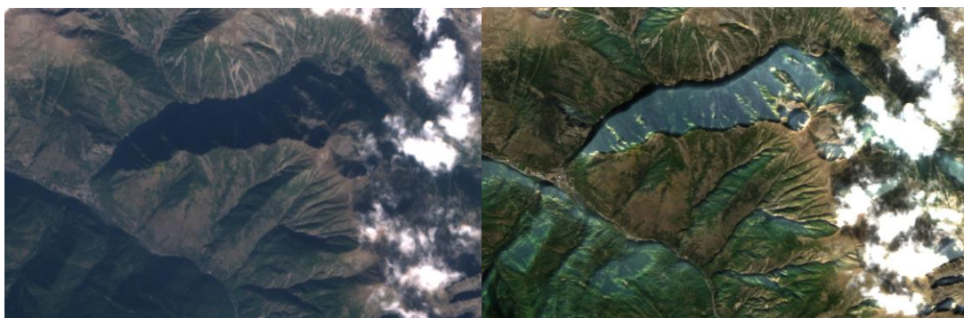
Figure 5-3: Terrain over-correction on shaded areas. Left: Level 1C true colour image, right: L2A true colour image.
