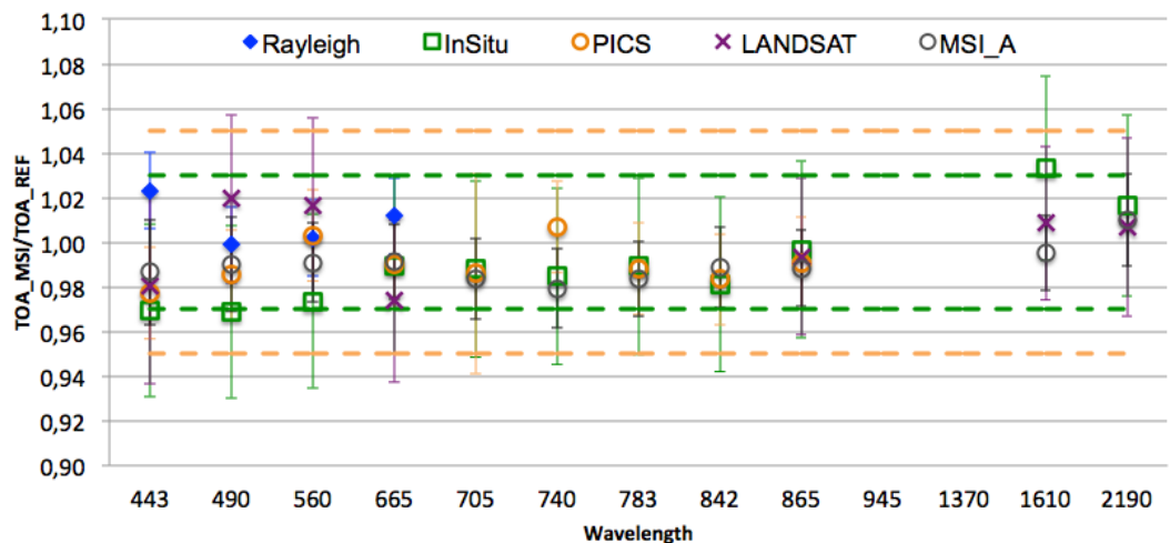
Figure 6: Comparison of radiometric accuracy for all spectral bands (except B09 & B10): ratio of S2B measurement on reference. Error bars indicate the method uncertainty.
