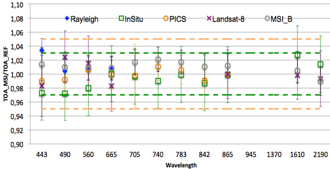
Figure 5: Comparison of radiometric accuracy for all spectral bands (except B09 and B10): ratio of S2A measurement on reference. Error bars indicate the method uncertainty.
