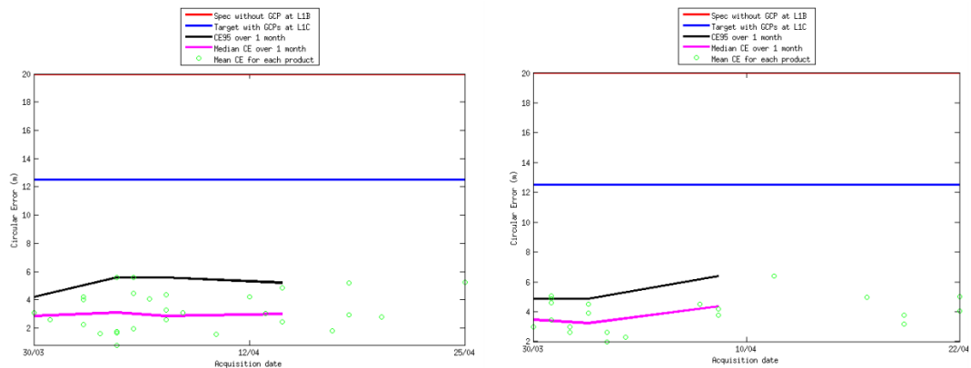
Figure 2: Absolute geolocation performance for refined products. Left: S2A, Right: S2B. The median (purple curve) and 95.45% confidence (black curve) performances are computed over a sliding window of 30 days. (07/05/2021).
