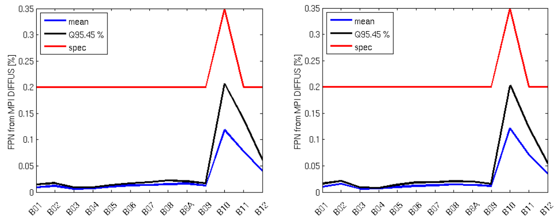
Figure 8: Fixed Pattern Noise (residual error after equalization) measured on diffuser images for S2A (left) and S2B (right). Blue curve: mean FPN, black: 95 percentile, red: specified value.
