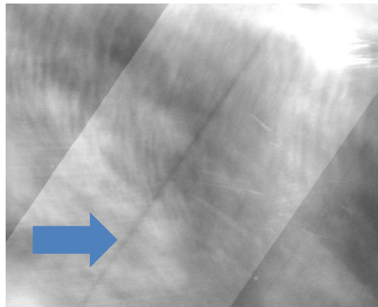
Figure 26: Along-track stripe on B11 image due to a non-linear response on D11 (contrast strongly enhanced).
