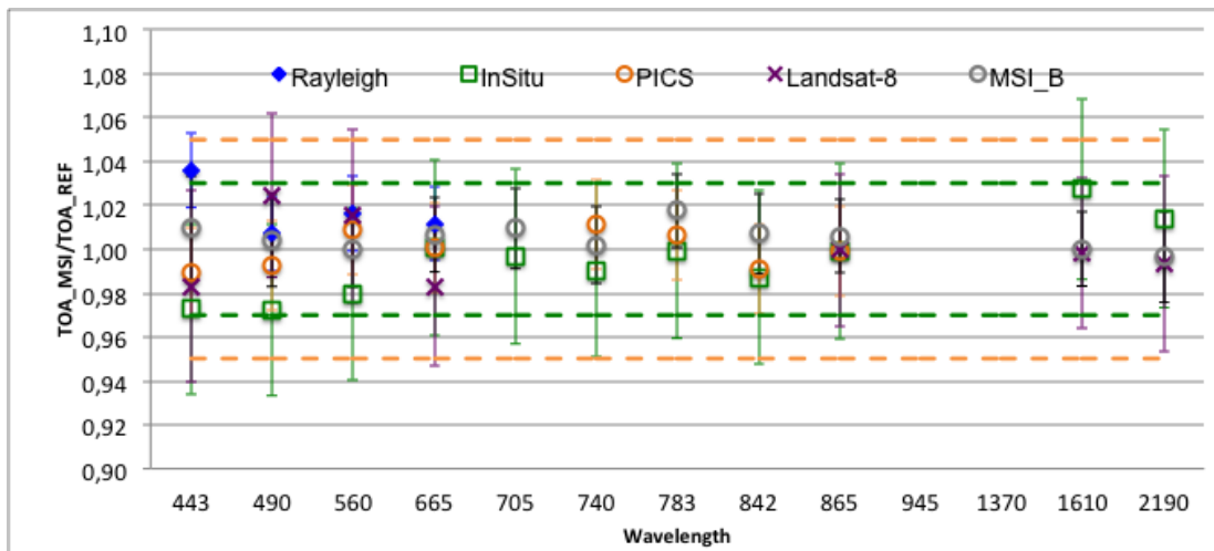
Figure 3: Comparison of radiometric accuracy for all spectral bands (except B09 and B10): ratio of S2A measurement on reference. Error bars indicate the method uncertainty.
