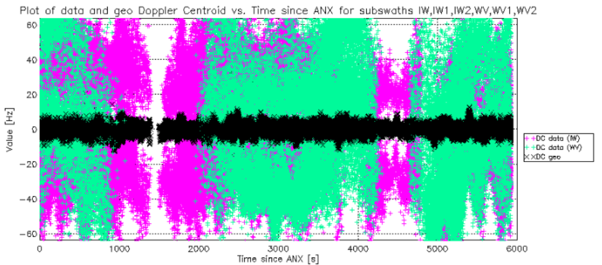
Figure 8 S1-A Doppler Centroid as respect to 1) time (vertical black lines representing the date of manoeuvres) and 2) ANX time (top and bottom respectively cycle 313-314 and cycles 315-316)
