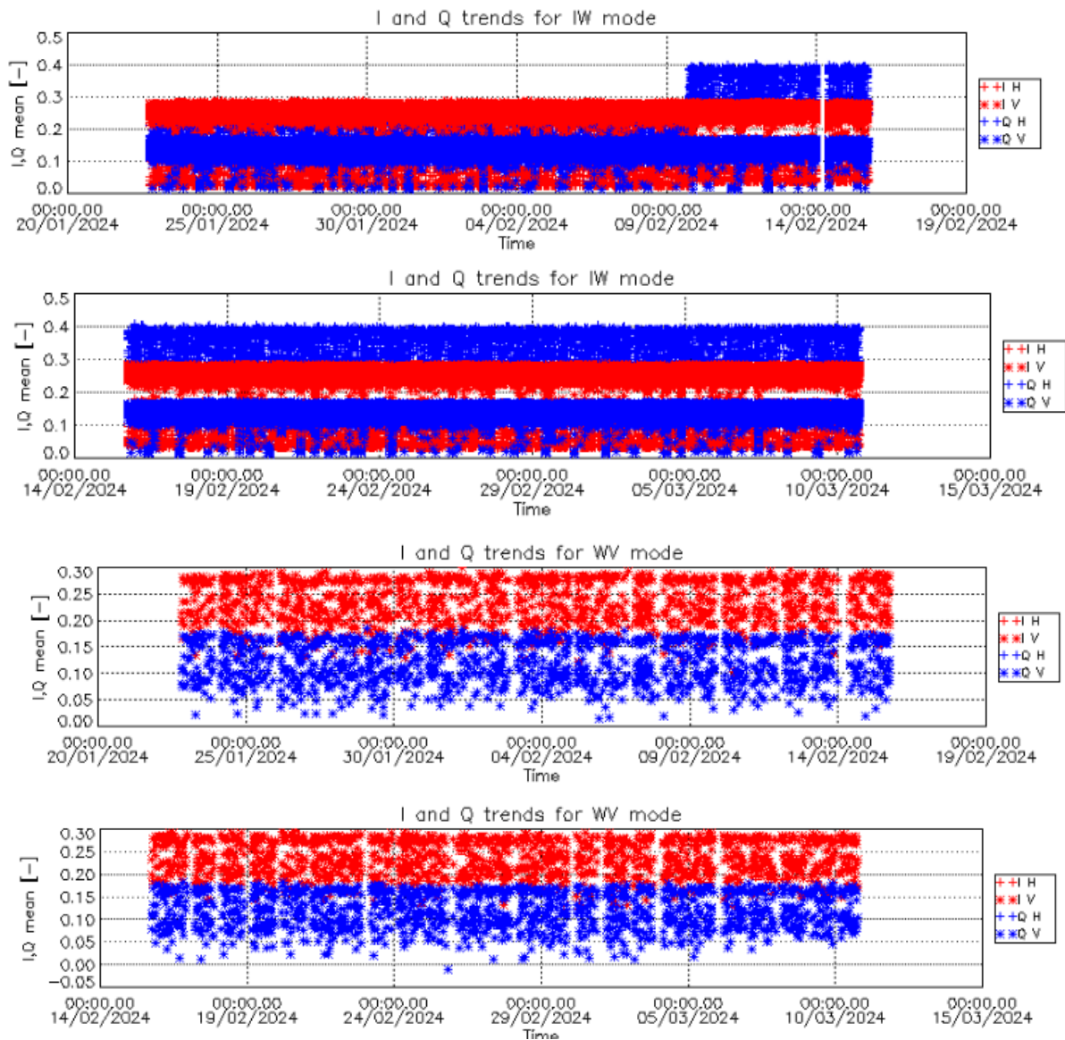
Figure 2 I&Q Channels
