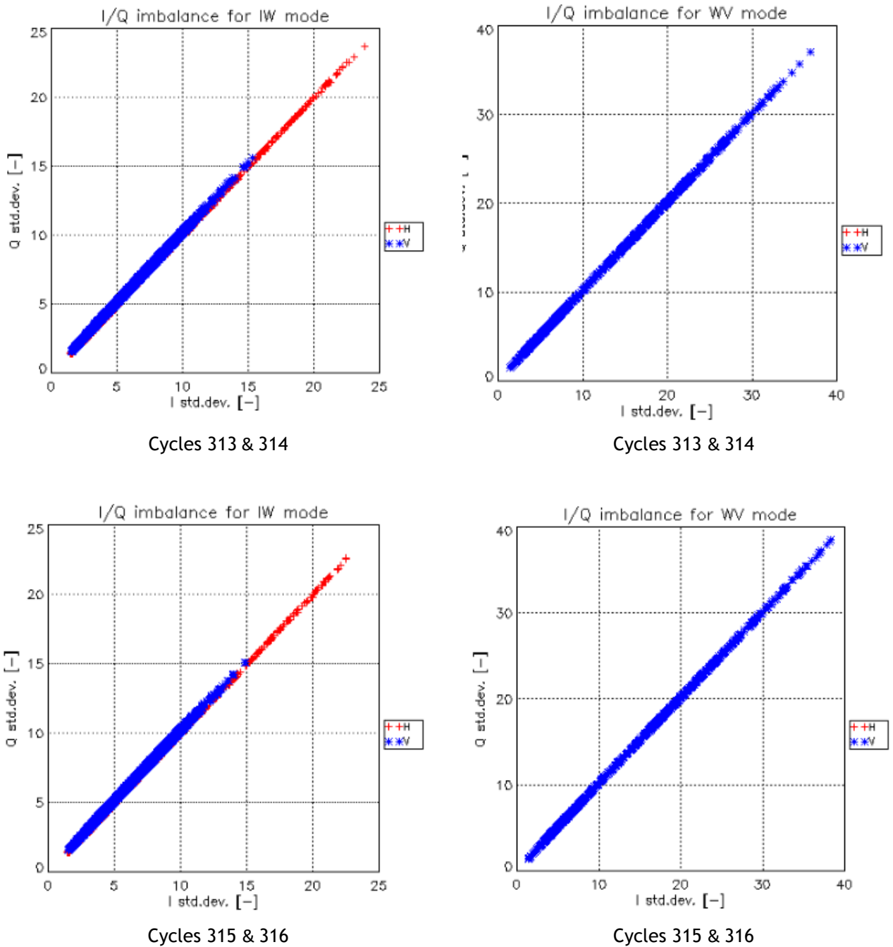
Figure 3 WV I&Q Channel Imbalance
