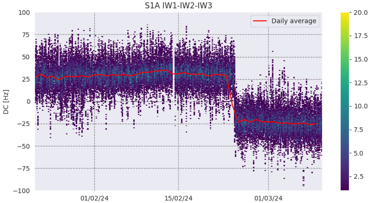
Figure 9 Sentinel1-A Doppler Centroid two-dimensional histogram. Red line shows average on a daily basis. Colour bar shows number of observations for each date-DC bin.
