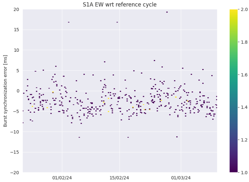
Figure 10: Burst synchronization error for current reporting period, monitoring with respect to reference cycle.
