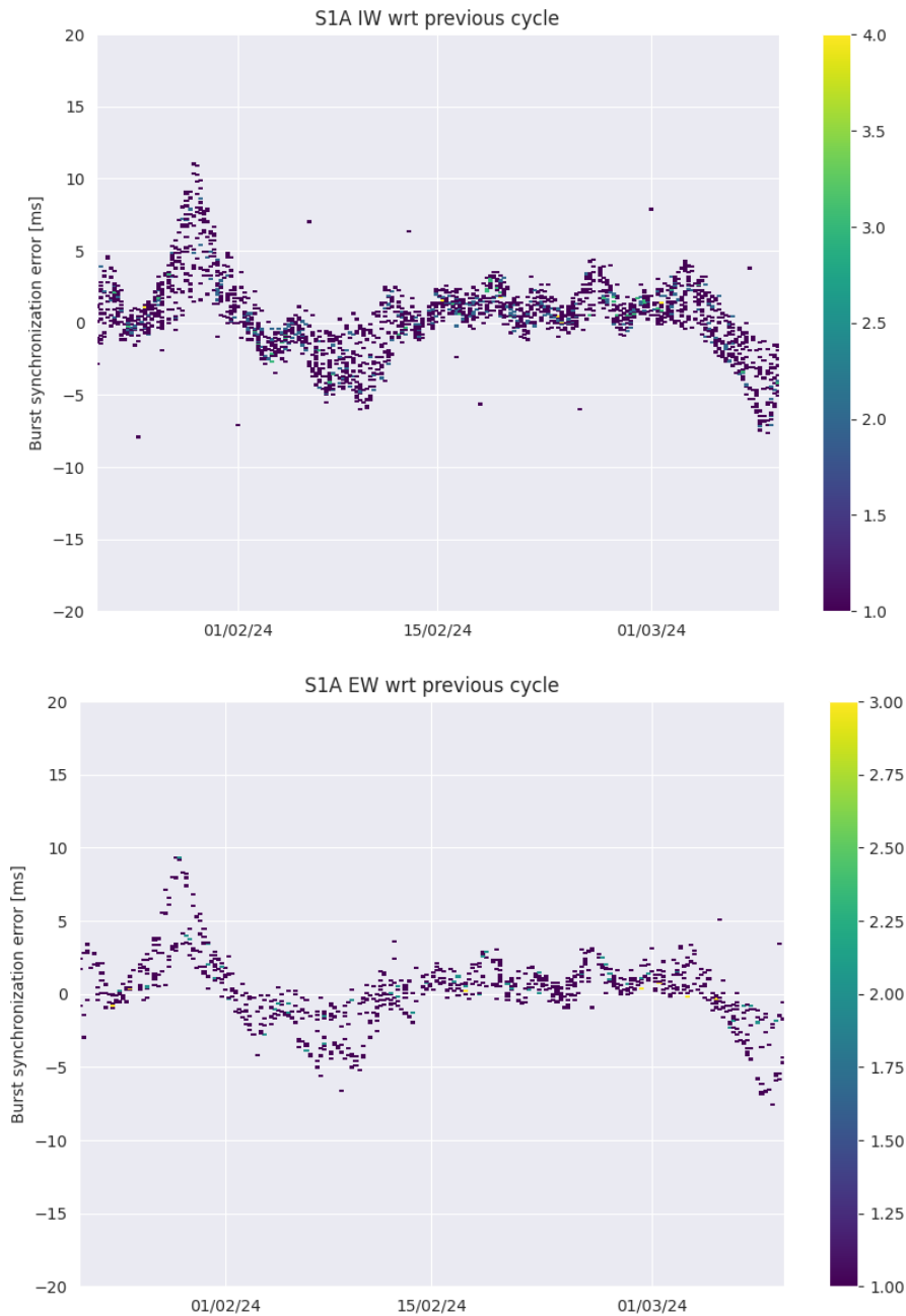
Figure 11 Burst synchronization error for current reporting period, monitoring with respect to previous cycle.
