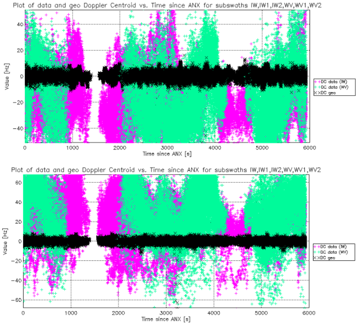
Figure 8 S1-A Doppler Centroid as respect to 1) time (vertical black lines representing the date of manoeuvres) and 2) ANX time (top and bottom respectively cycle 301-302 and cycles 303-304)
