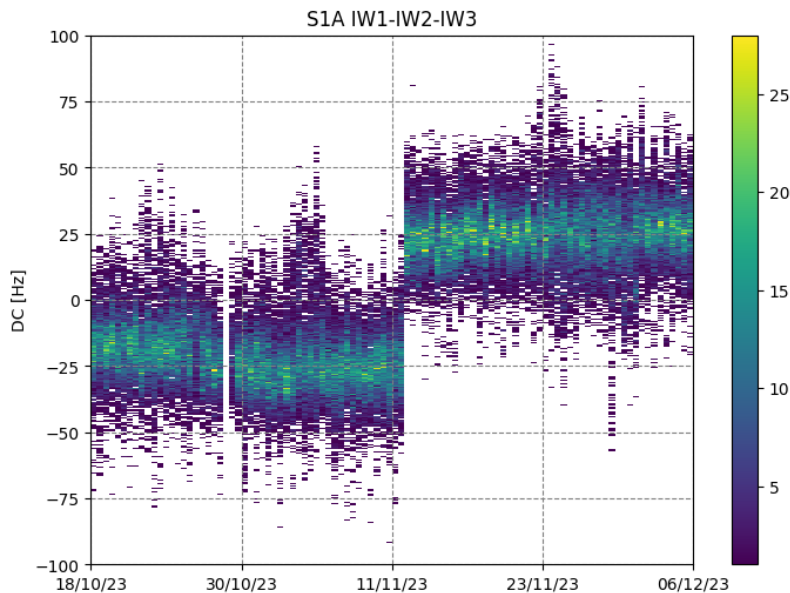
Figure 9 S1-A Doppler Centroid
