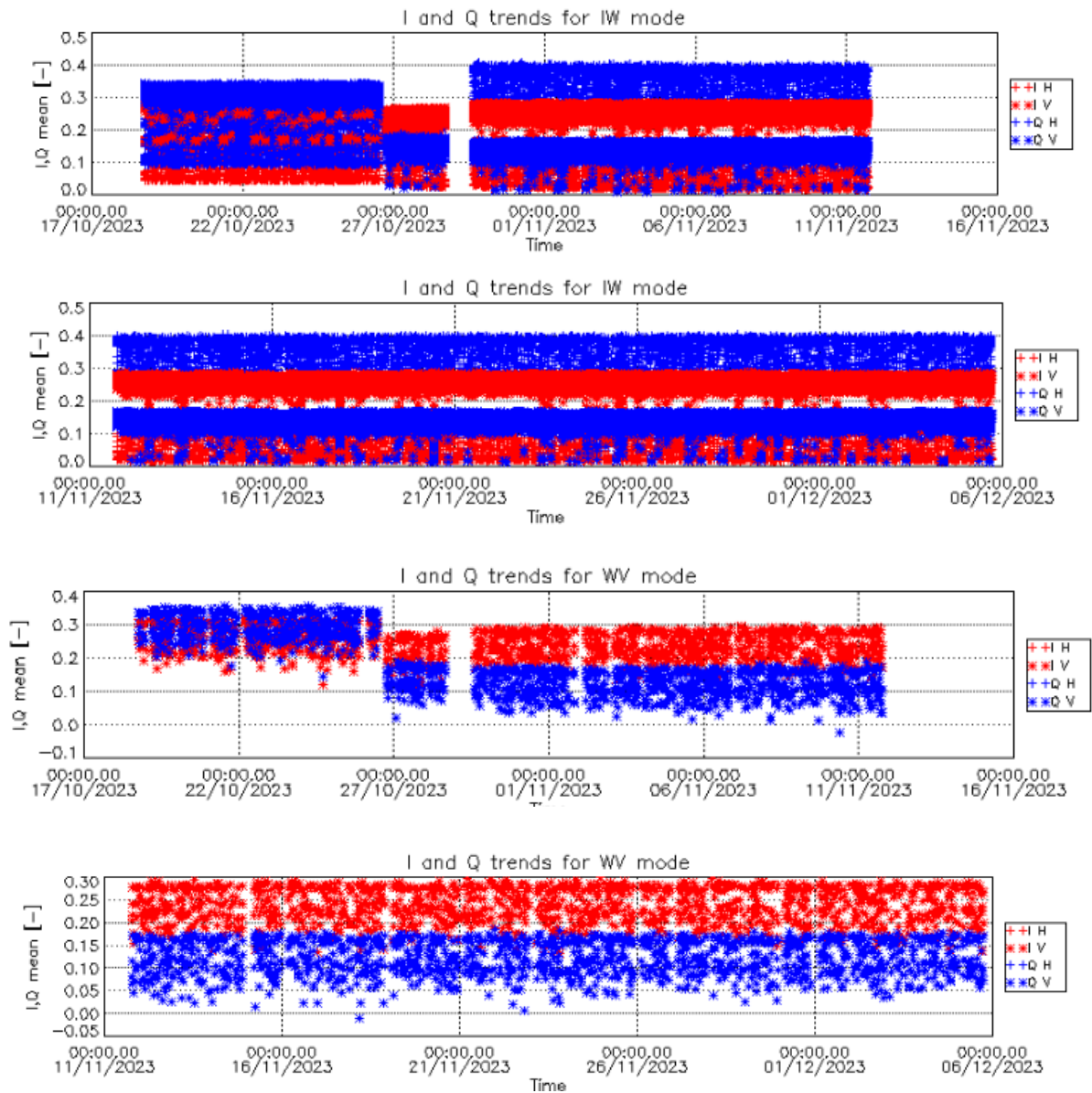
Figure 2 I&Q Channels
