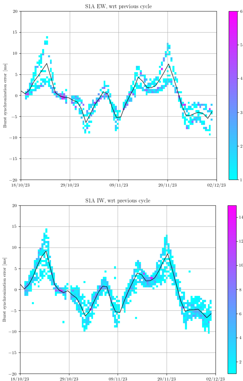
Figure 11 Burst synchronization error for current reporting period, monitoring with respect to previous cycle.
