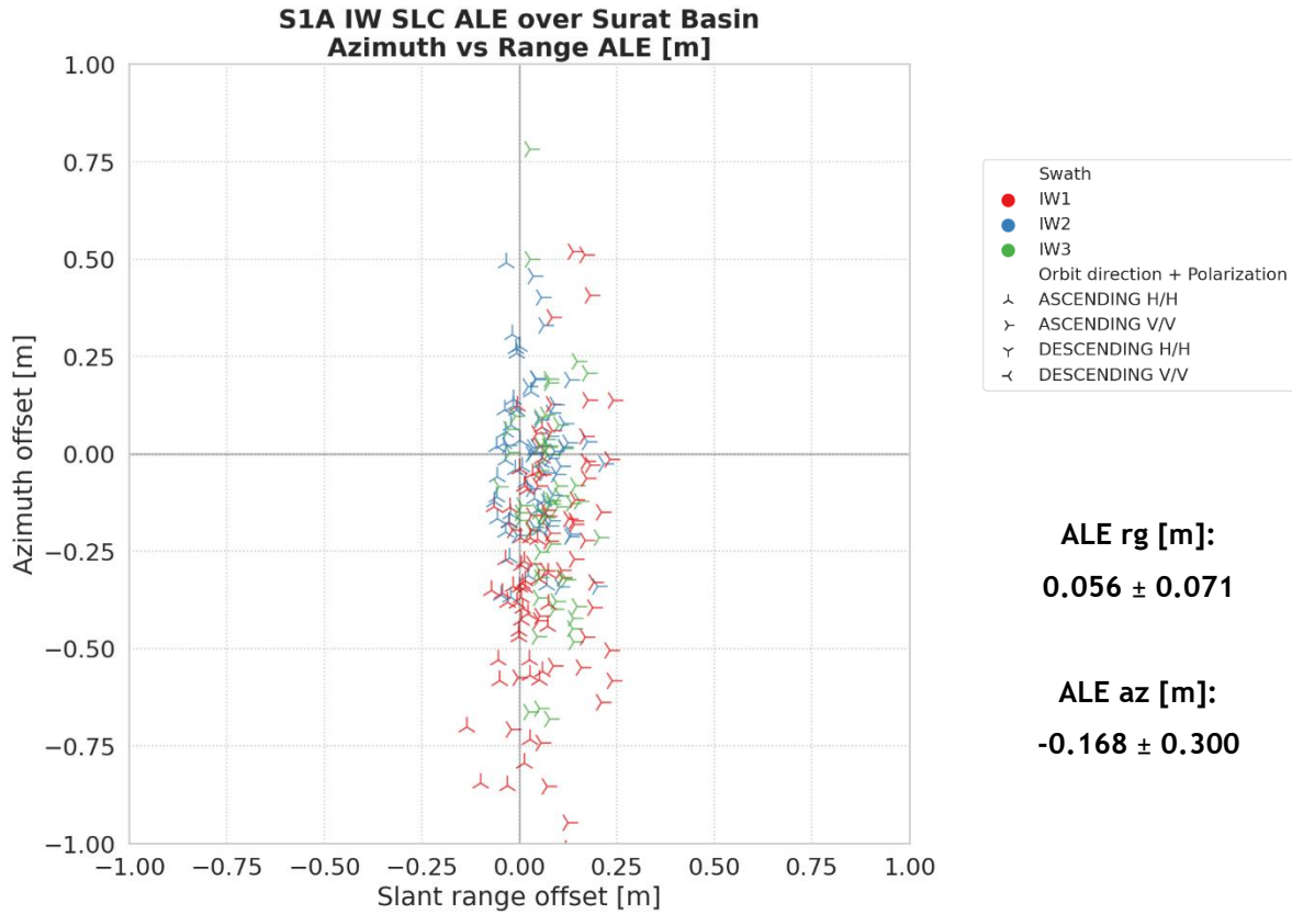
Figure 6 S1-A absolute localisation error based on S-1A IW SLC products acquired over the Surat Basin test site during the current reporting period (18 Oct to Dec 5, 2023).
