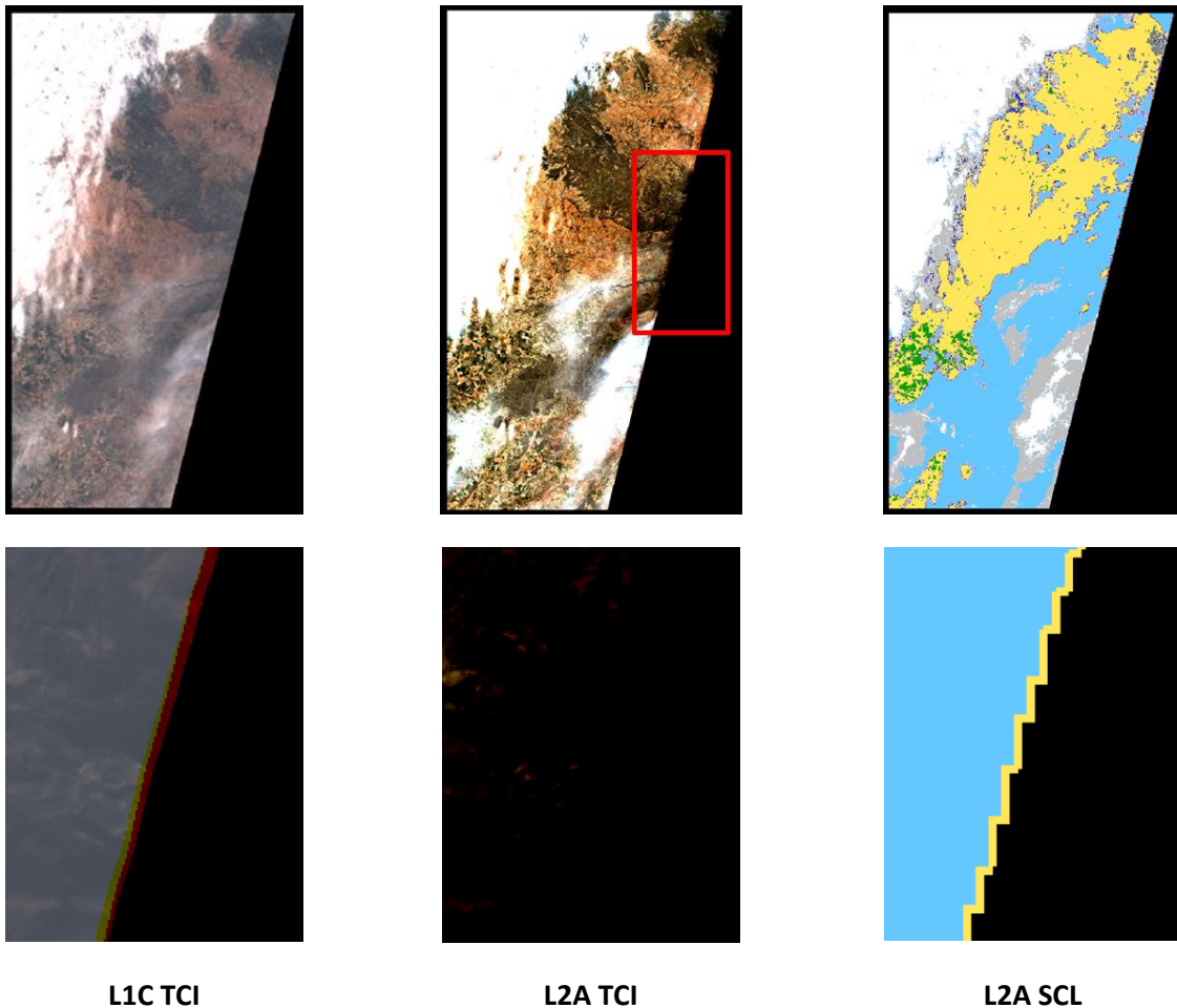
Figure 5 : Illustration of the very low negative reflectances near the edge of the swath observed on the L2A product: S2B_MSIL2A_20220329T105629_N0400_R094_T30SXJ_20220329T134242. An illustration of the corresponding L1C product (first column) is also shown
