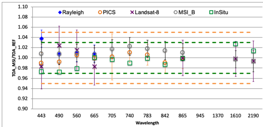
Figure 8: Comparison of radiometric accuracy for all spectral bands (except B09 and B10): ratio of S2A measurement on reference. Error bars indicate the method uncertainty. Updated over Rayleigh and PICS up to 4/2022
