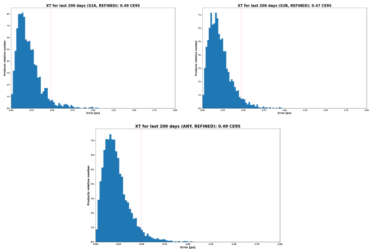
Figure 6: Multi-temporal 2D co-registration errors for refined S2A (left) and S2B pairs (right), and all pairs (bottom) on 08/2022. The 95.45% performance is <5 m.
