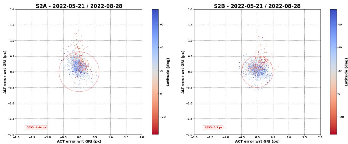
Figure 4: Absolute geolocation performance for refined products. Left: S2A, Right: S2B (21.05.2022 – 28.08.2022)
