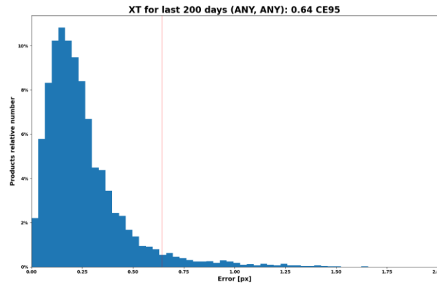
Figure 7: Histogram of the multi-temporal performance for all products (refined and unrefined) – 08/2022
