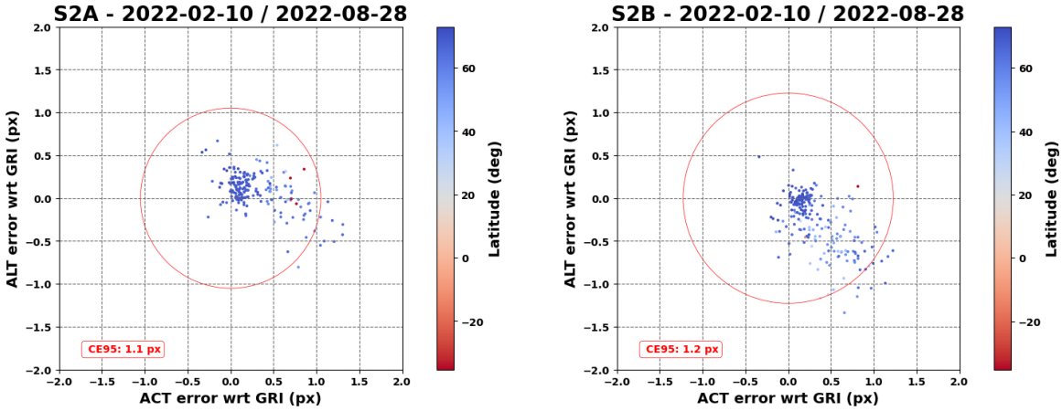
Figure 1: Absolute geolocation performance for unrefined products. Left: S2A, Right: S2B (06.01.2022 – 24.07.2022)
