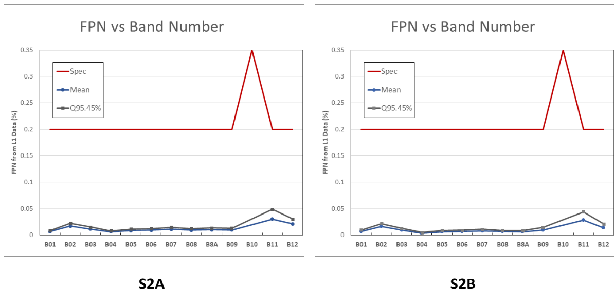
Figure 14 : Fixed Pattern Noise (residual error after equalization) measured on homogeneous natural images for S2A (left) and S2B (right) from 06/2022 to 07/2022. Blue curve: mean FPN, grey curve: Q95.45 percentile, red curve: specified value.
