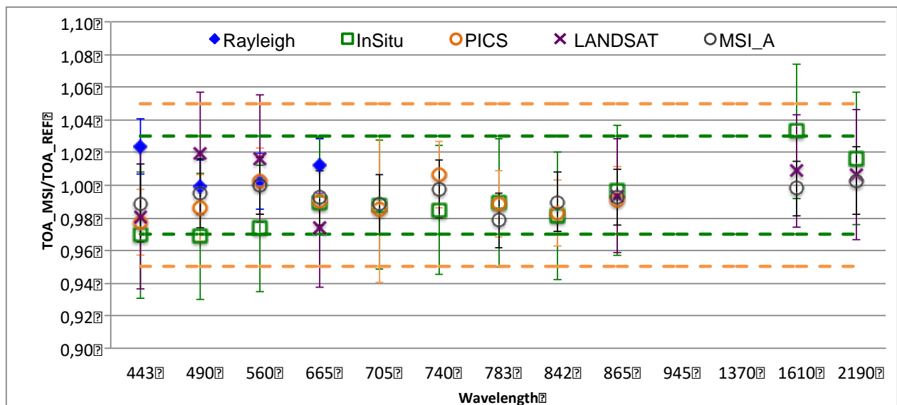
Figure 7: Comparison of radiometric accuracy for all spectral bands (except B09 & B10): ratio of S2B measurement on reference. Error bars indicate the method uncertainty. 12/2021
