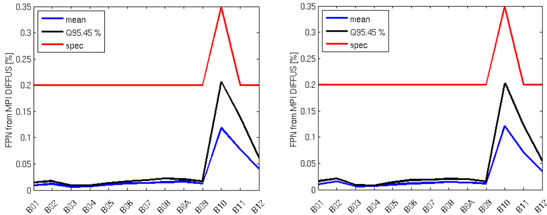
Pattern Noise (residual error after equalization) measured on diffuser images for S2A (left) and S2B (right). Blue curve: mean FPN, black: 95 percentile, red: specified value.
