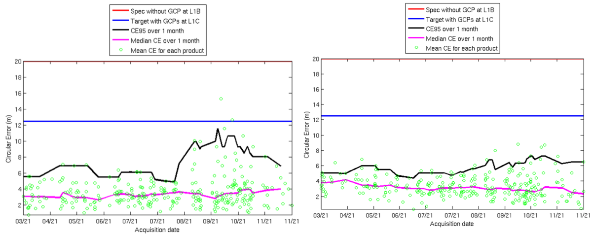
Figure 3: Absolute geolocation performance for refined products. Left: S2A, Right: S2B. The median (purple curve) and 95.45% confidence (black curve) performances are computed over a sliding window of 30 days. (01/2022).
