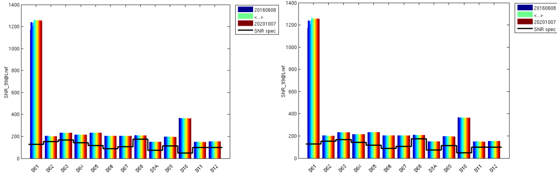
Figure 8: Evolution of the SNR performances on S2A since 08/06/2016 (left) and S2B since 15/03/2017 (right)
