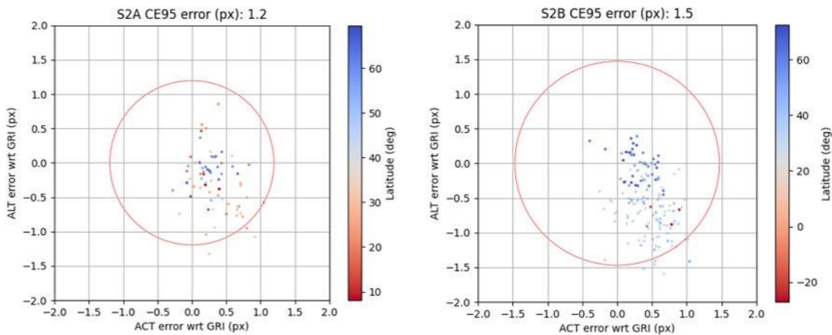
Figure 1: Absolute geolocation performance for unrefined products. Left: S2A, Right: S2B (04.2021 – 01.2022)
