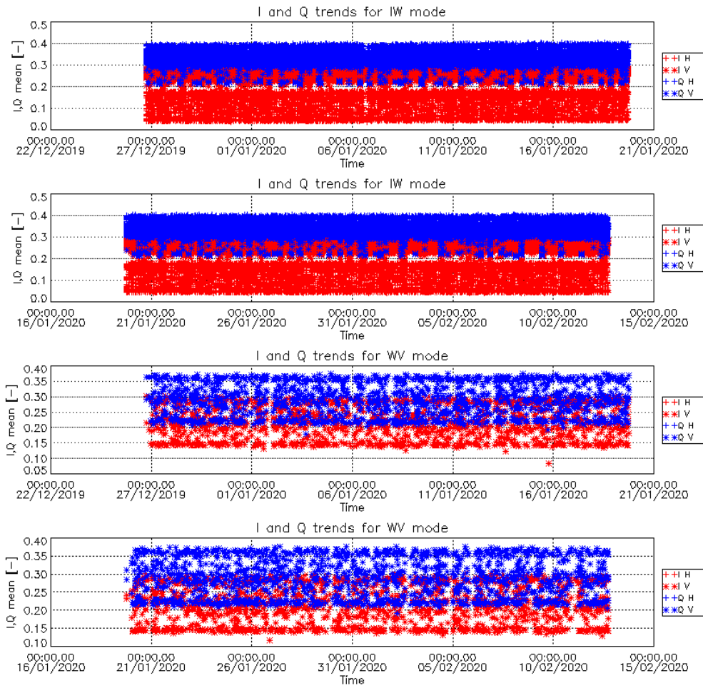
Figure 2 I&Q Channels
