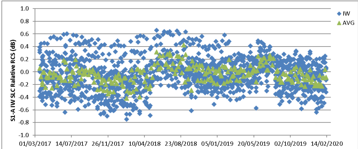
Figure 6 IW Long-Term Relative Radar Cross-Section
