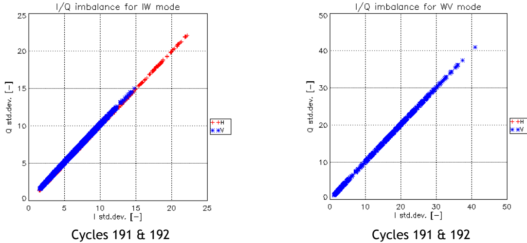
Figure 3 WV I&Q Channel Imbalance
