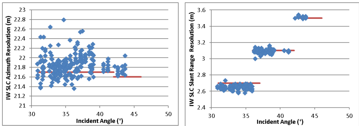
Figure 4 IW Azimuth and Slant Range Spatial Resolutions
