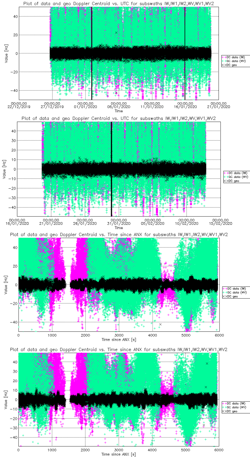
Figure 8 S1-A Doppler Centroid
