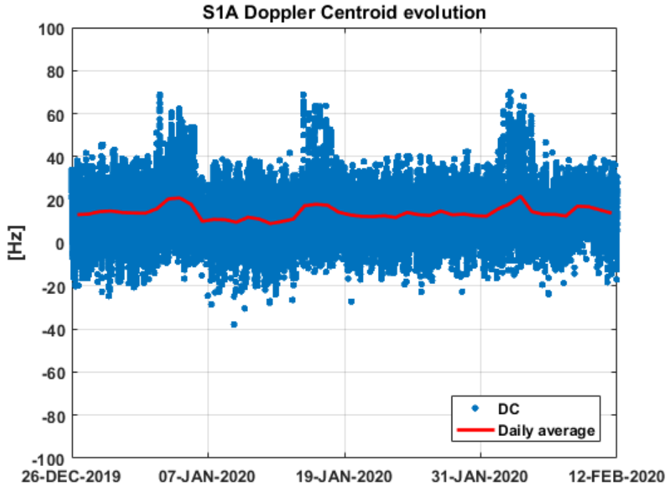
Figure 9 S1-A Doppler Centroid
