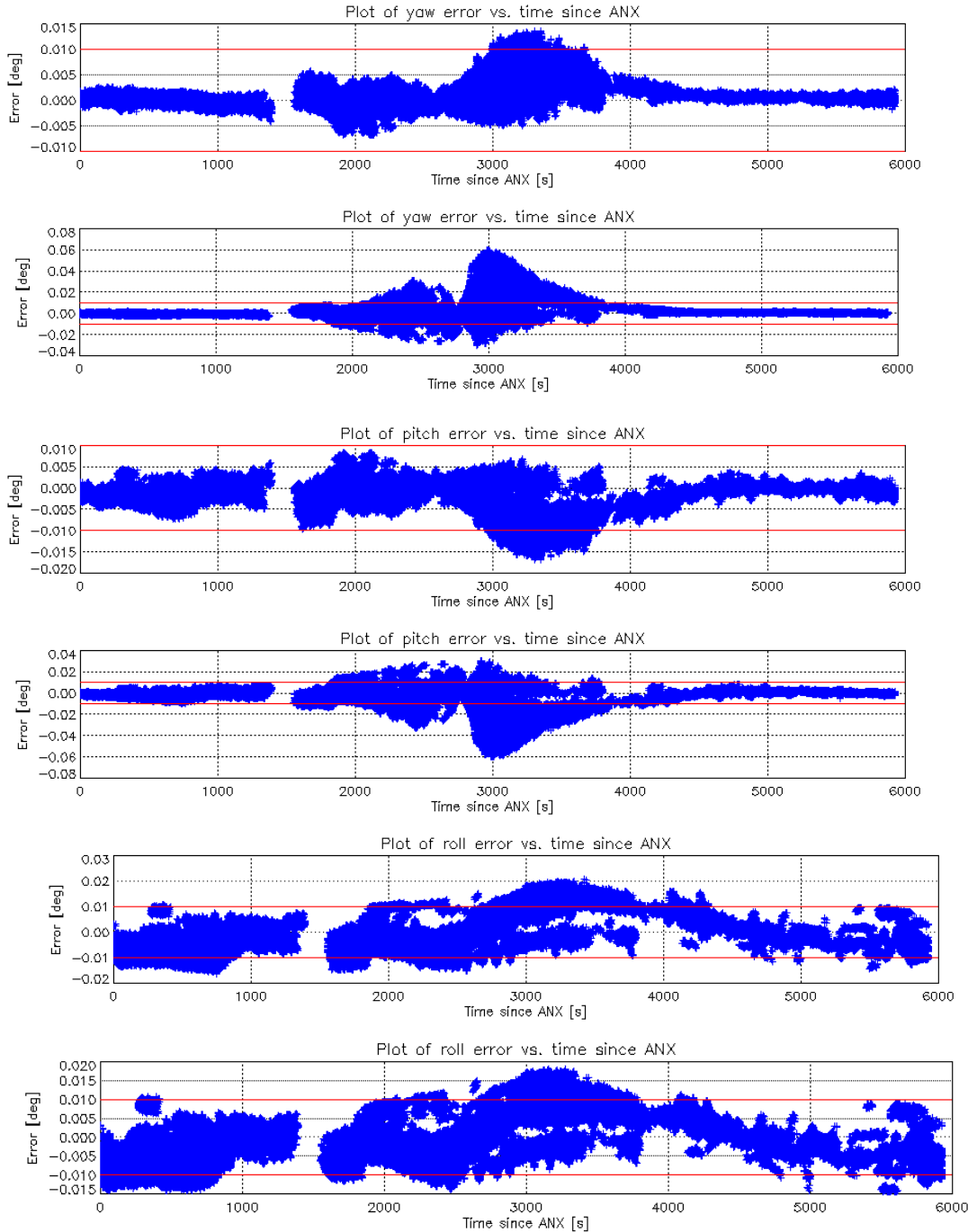
Figure 7 S1-A Yaw, Pitch and Roll Errors
