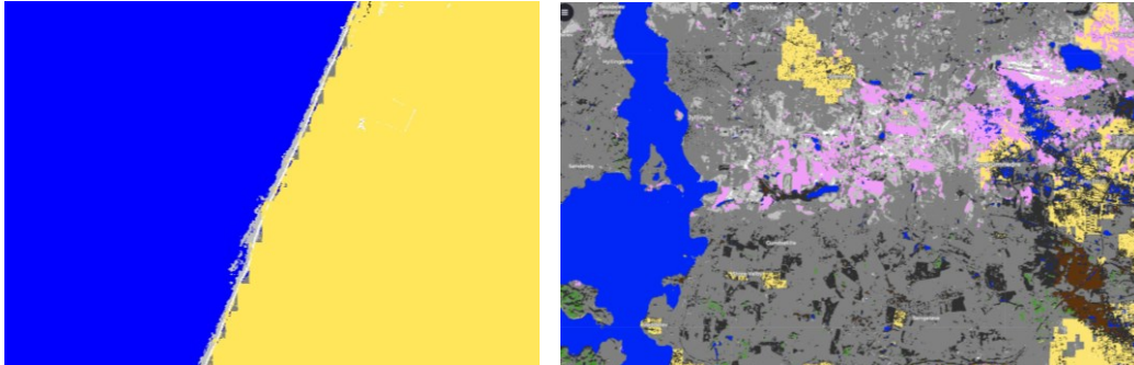
Figure 12: Blocky patterns on the scene classification layer (SCL). Left: near the coastline. Right: near city boundaries.
