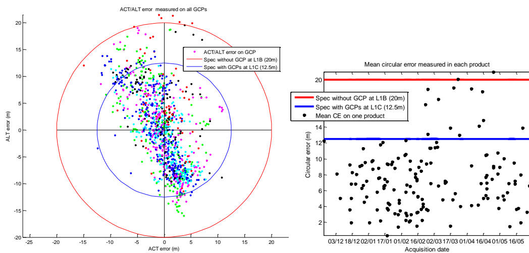
Figure 2: Geolocation performance assessment. Left: Statistics of the geolocation error for all Ground Control Points analysed during the reporting period. Right: Evolution of the measured performance.
