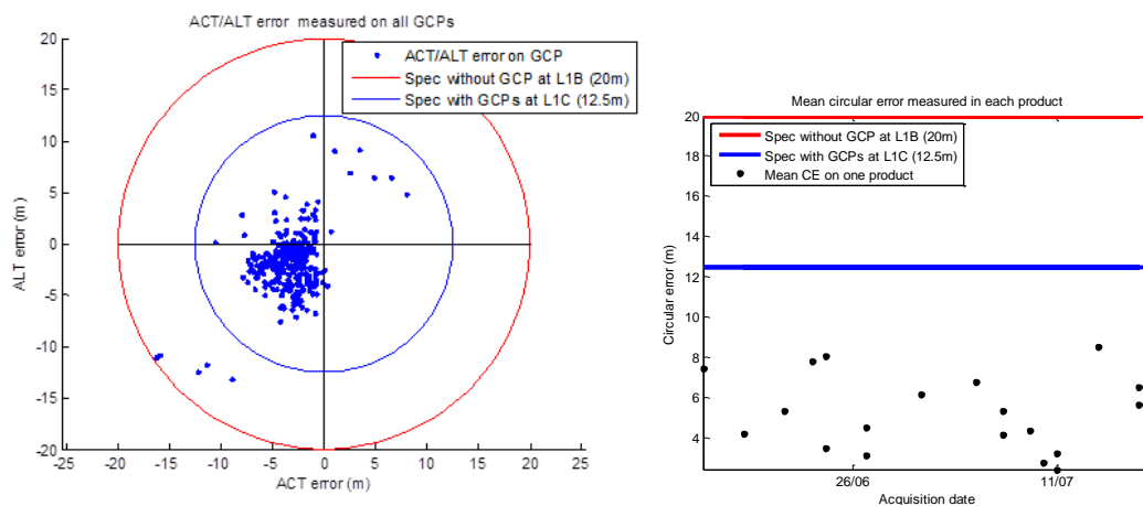
Figure 3: Geolocation performance assessment with processing baseline 02.04. Left and Right: same legend as in Figure 2 above.
