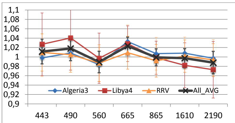
Figure 3: Ratio of S2 MSI to LANDSAT OLI TOA reflectances acquired in similar viewing conditions. Sites Algeria3, Lybia4, Railroad Valley and average value. Error bars indicate the uncertainty of the methodology.
