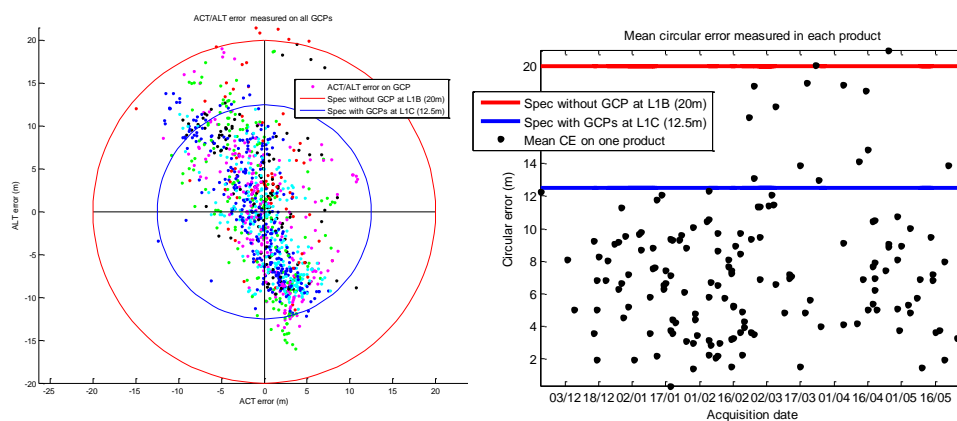
Figure 1: Geolocation performance assessment. Left: Statistics of the geolocation error for all Ground Control Points analysed during the reporting period. Right: Evolution of the measured performance.
