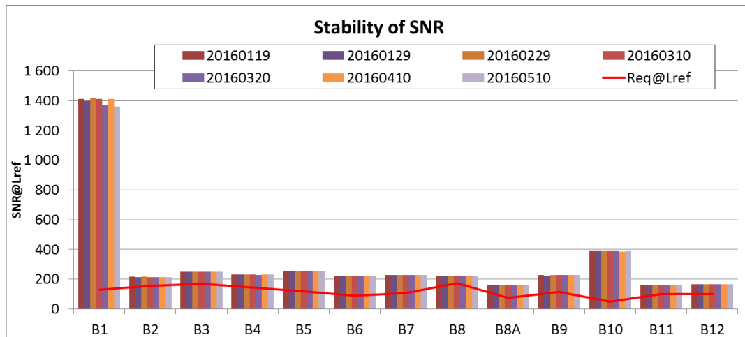
Figure 4: Evolution of the SNR performance since 19/01/2016.
