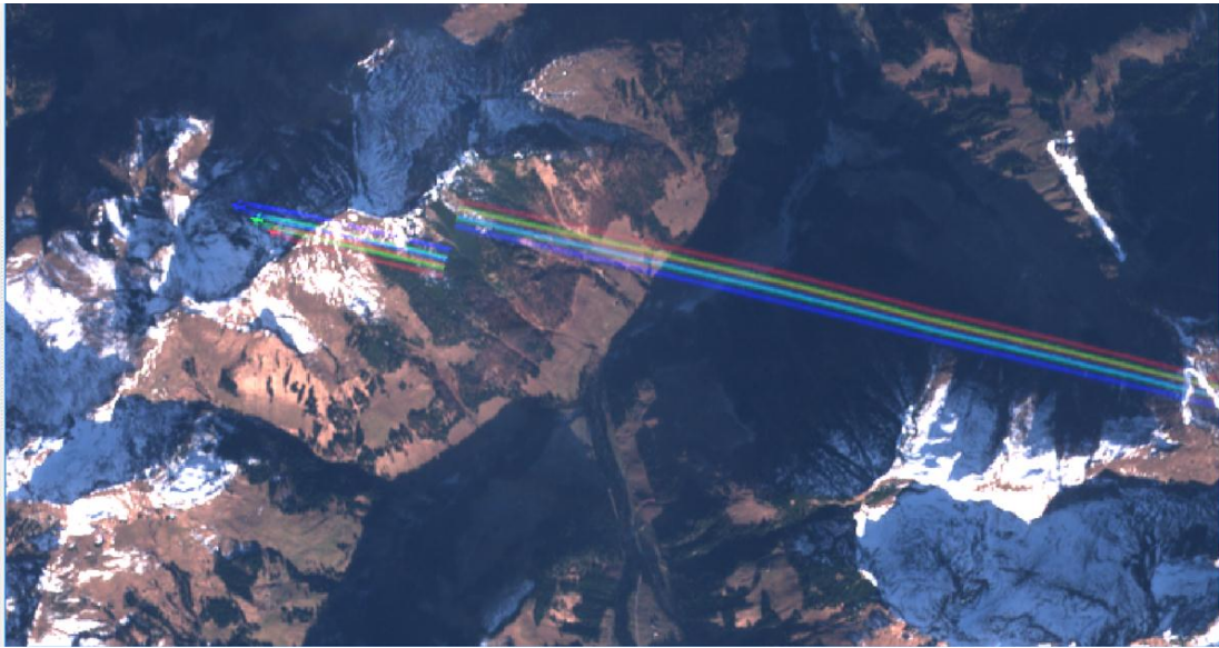
Figure 10: Spectral mis-registration and detector misalignment for object at high altitude (plane and contrail). This feature is not an anomaly.
