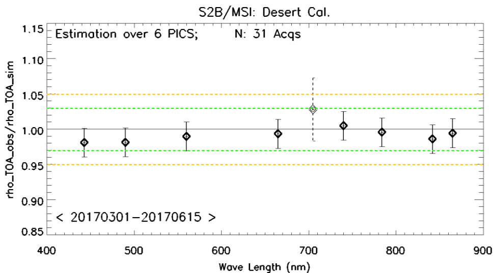
Figure 5: Radiometric accuracy estimation for S2B using the PICS method for bands B01 to B8A. Ratio of S2B measurement on reference. Errors bars indicate the method uncertainty.
