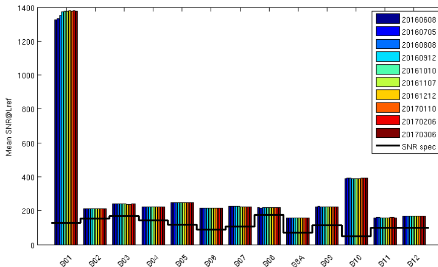
Figure 5: Evolution of the SNR performance since 06/08/2016.
