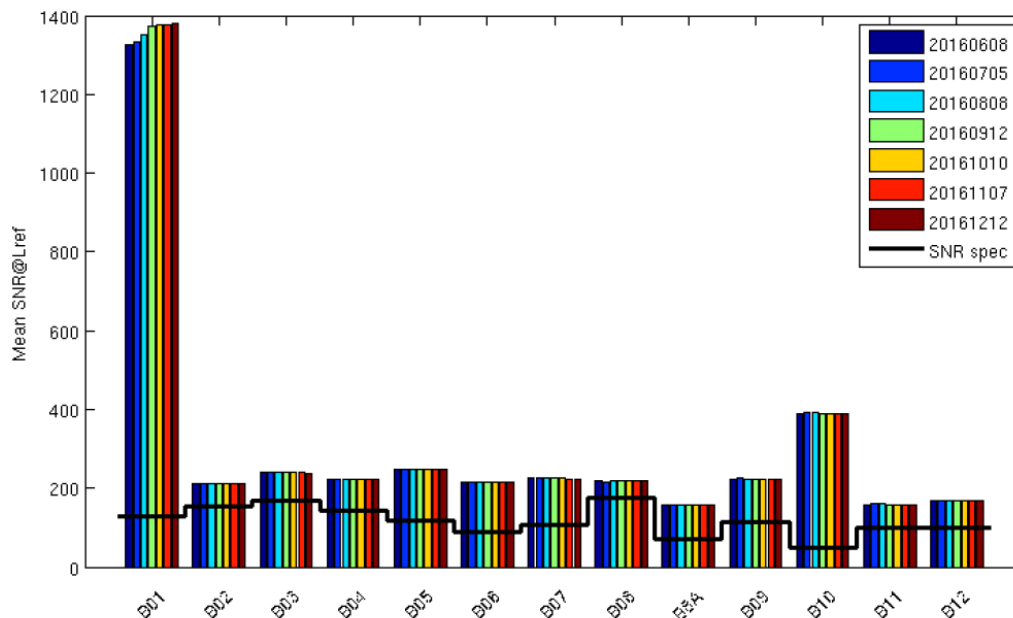
Figure 5: Evolution of the SNR performance since 06/08/2016.
