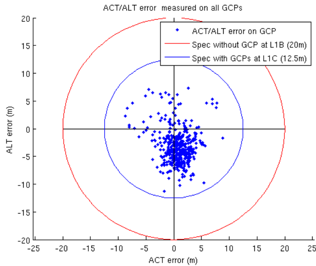
Figure 1: Geolocation performance measured on 68 products since 15/11/2106 (for all Ground Control Points in Across-Track/Along-Track frame).
