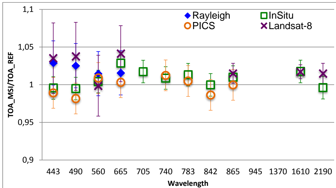
Figure 6: Comparison of radiometric accuracy for all spectral bands (except B10): ratio of S2A measurement on reference. Error bars indicate the method uncertainty.
