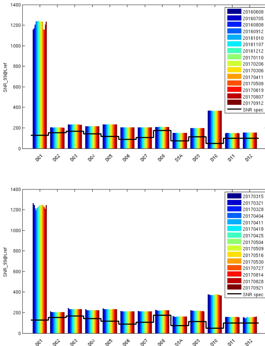
Figure 8: Evolution of the SNR performance or S2A since 08/06/2016 (top) and S2B since 15/03/2017 (bottom)
