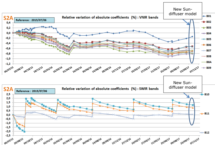
Figure 3: History of the absolute calibration coefficient for S2A. The last point has been computed with the new Sun-diffuser model. Variations for SWIR bands are correlated with instrument decontaminations.
