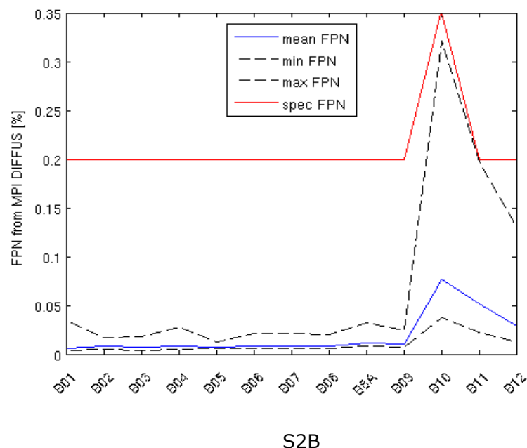
Figure 9: Fixed Pattern Noise (residual error after equalization) measured on diffuser images for S2A (top) and S2B (bottom). Blue curve: mean FPN, red: maximum specified value. Dashed: best- and worst-case pixels.
