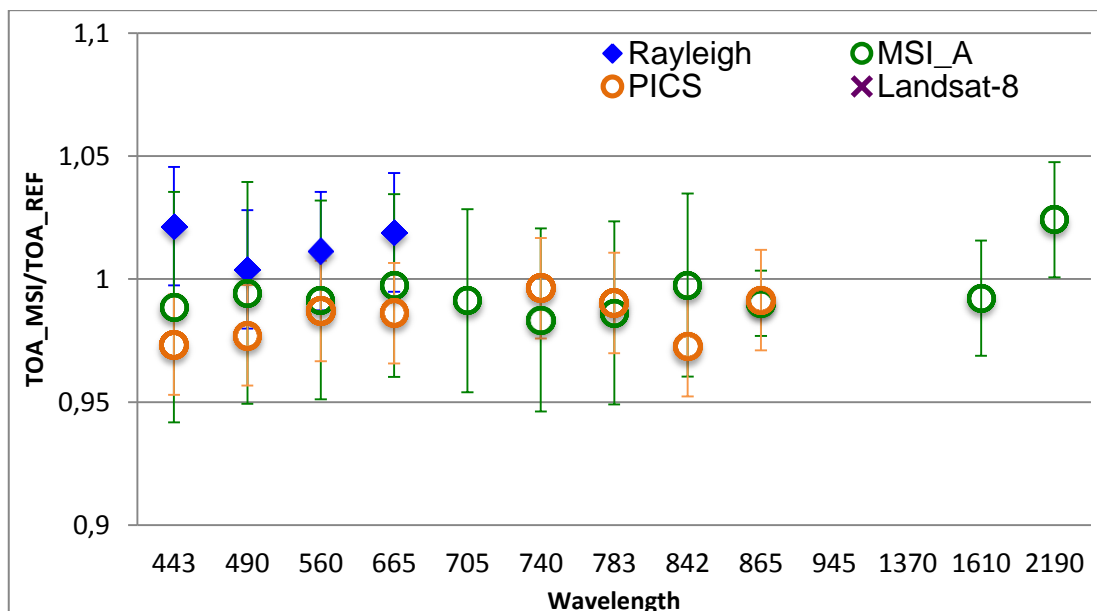
Figure 7: Comparison of radiometric accuracy for all spectral bands (except B09 & B10): ratio of S2B measurement on reference. Error bars indicate the method uncertainty.
