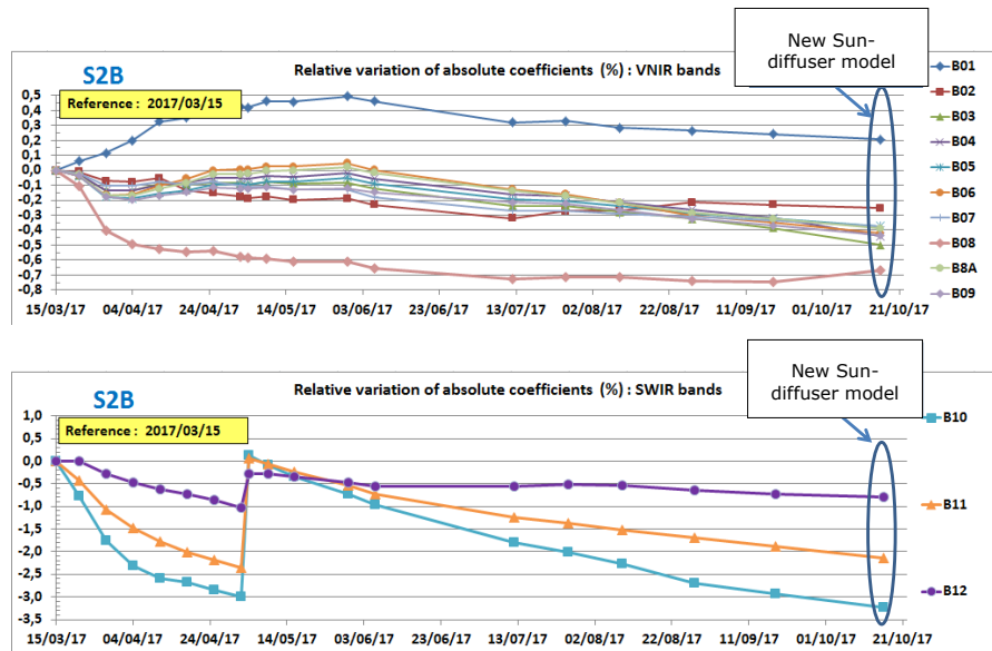
Figure 4: Same as above for S2B. Note the different time scale.
