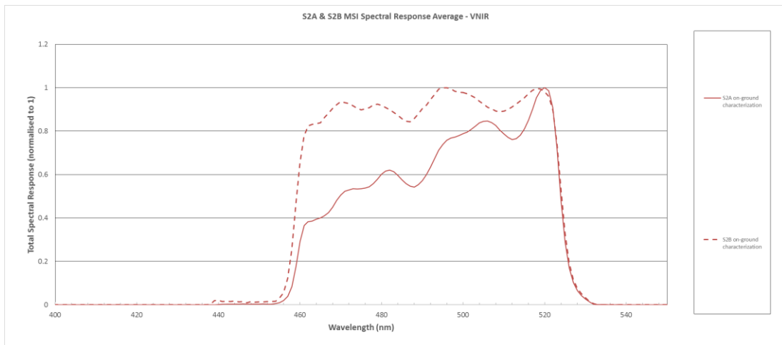
Figure 5: Comparison of S2A and S2B spectral response functions for band B02. Measurements for S2A (solid curve) are affected by a defect. Users are advised to consider measurements of S2B (dashed curve) for S2A instead.
