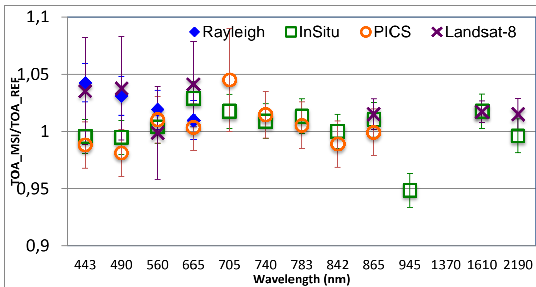
Figure 4: Comparison of radiometric accuracy for all spectral bands (except B10): ratio of S2A measurement on reference. Error bars indicate the method uncertainty.
