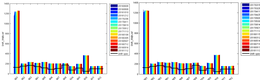
Figure 5: Evolution of the SNR performance on S2A since 08/06/2016 (left) and S2B since 15/03/2017 (right)
