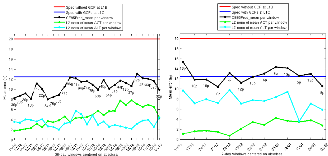
Figure 1: Geolocation performance for S2A (left) and S2B (right). The performance is computed over a sliding window of 30 days (S2A, left) or 7 days (S2B, right). Number of products used in the sliding window indicated for each point. (ACT= across track, ALT= along track). A vertical line indicates a geometric calibration event.
