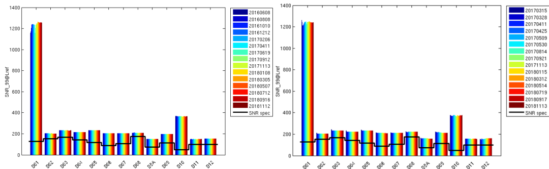
Figure 5: Evolution of the SNR performance of S2A since 08/06/2016 (left) and S2B since 15/03/2017 (right)
