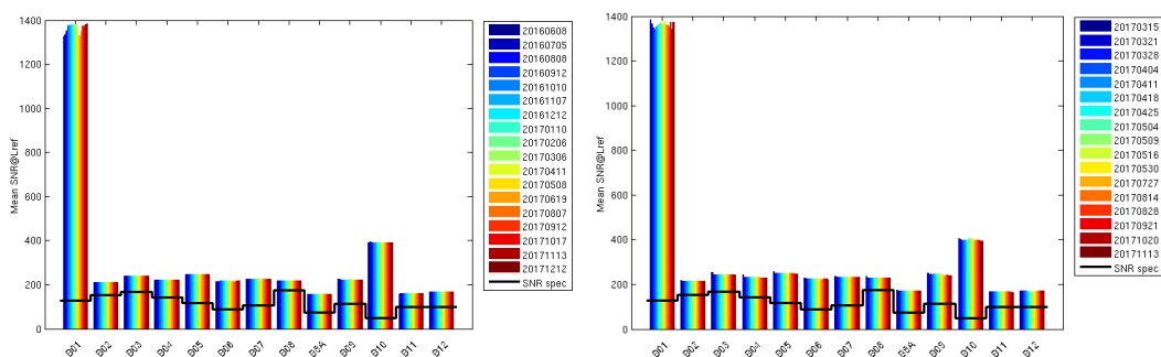
Figure 6: Evolution of the SNR performance for S2A since 08/06/2016 (left) and S2B since 15/03/2017 (right)
