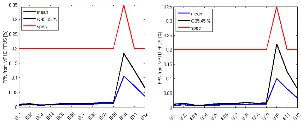
Figure 7: Fixed Pattern Noise (residual error after equalization) measured on diffuser images for S2A (left) and S2B (right). Blue curve: mean FPN, black: 95 percentile, red: specified value.
