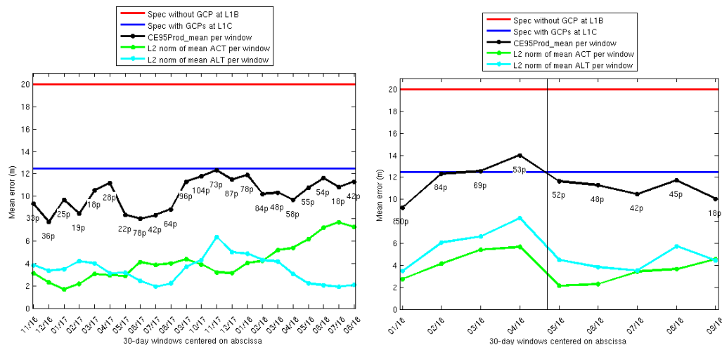
Figure 1: Geolocation performance for S2A (left) and S2B (right). The performance is computed over a sliding window of 30 days. Number of products used in the sliding window indicated for each point. (ACT= across track, ALT = along track). A vertical line indicates a geometric calibration event.
