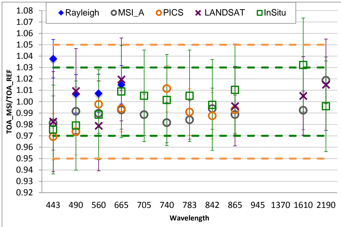
Figure 5: Comparison of radiometric accuracy for all spectral bands (except B09 & B10): ratio of S2B measurement on reference. Error bars indicate the method uncertainty.
