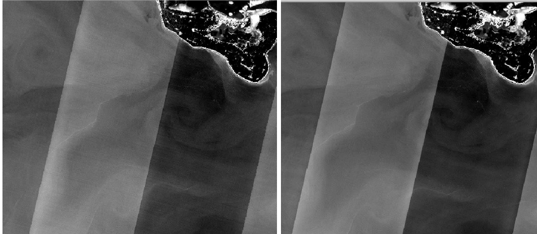
Figure 10: B01 image over sea with the current processing baseline 02.06 (Left) and the new processing baseline 02.07 (Right). Across-track lines due to correlated dark signal noise have been filtered.
