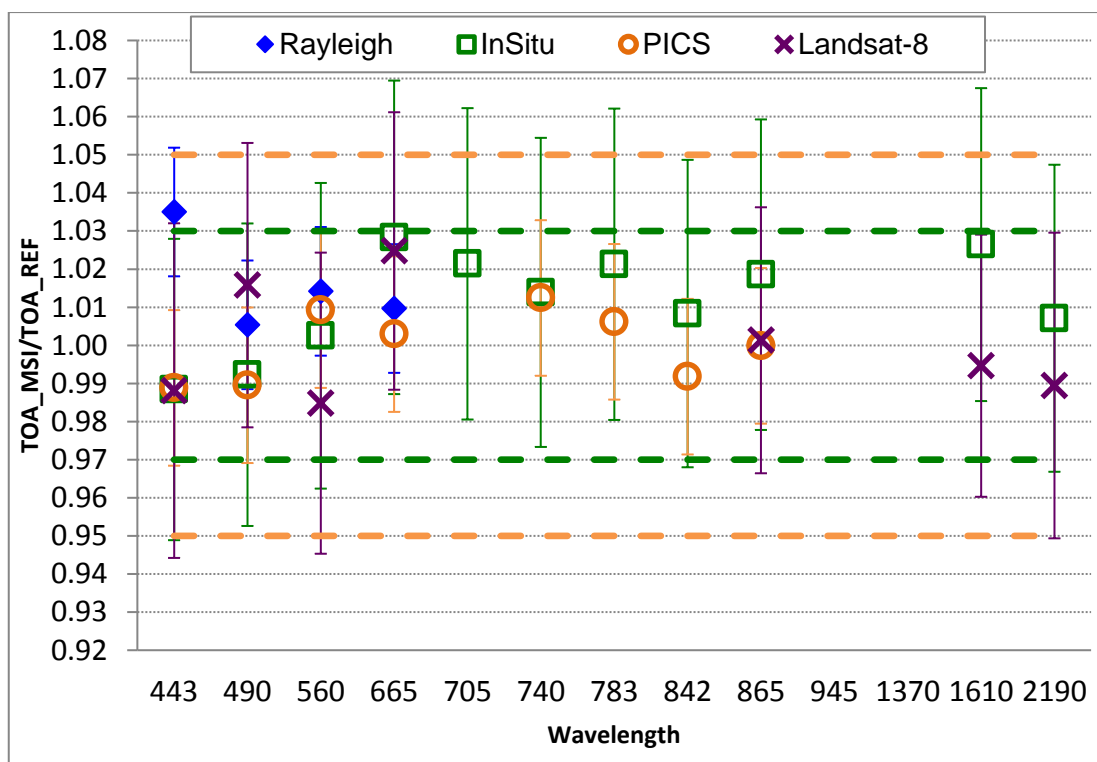
Figure 4: Comparison of radiometric accuracy for all spectral bands (except B10 and B09): ratio of S2A measurement on reference. Error bars indicate the method uncertainty.
