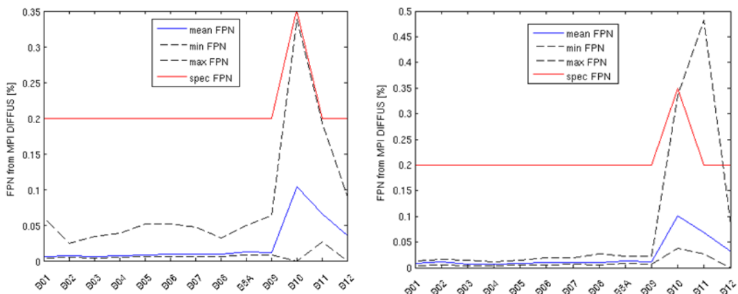
Figure 7: Fixed Pattern Noise (residual error after equalization) measured on diffuser images for S2A (left) and S2B (right). Blue curve: mean FPN, red: maximum specified value. Dashed: best- and worst-case pixels.
