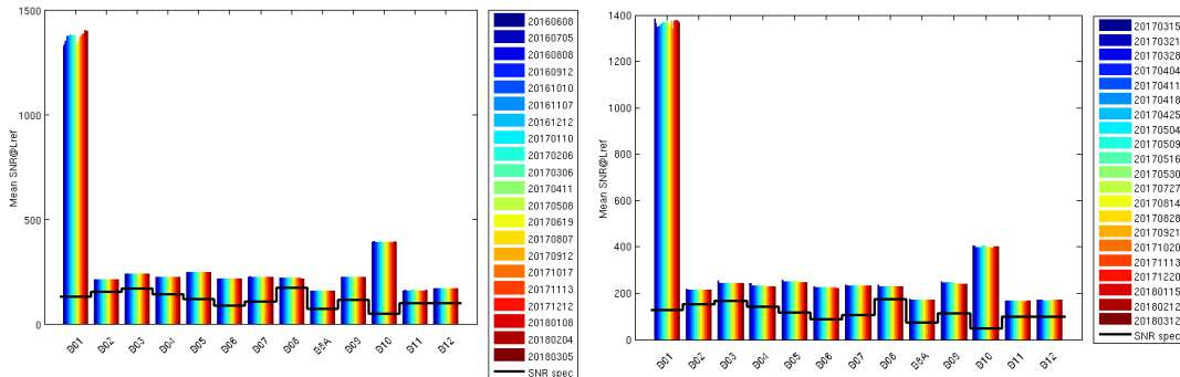
Figure 6: Evolution of the SNR performance or S2A since 08/06/2016 (left) and S2B since 15/03/2017 (right)
