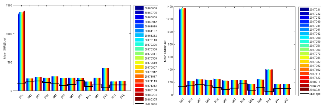
Figure 6: Evolution of the SNR performance of S2A since 08/06/2016 (left) and S2B since 15/03/2017 (right)
