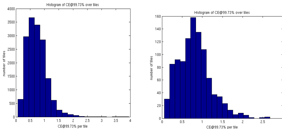
Figure 2: Histogram of the multi-temporal performance for S2A (left) and S2B (right, different scale). The 3 m requirement will be applicable only after activation of the geometrical refinement. The current performance is 11 m (S2A) and 14 m (S2B) at 95% confidence.
