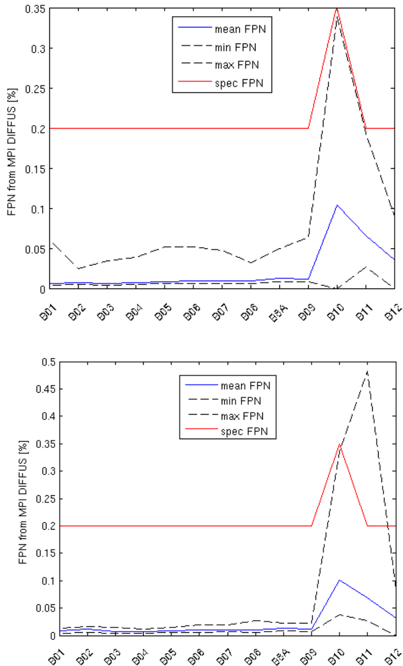
Figure 7: Fixed Pattern Noise (residual error after equalization) measured on diffuser images for S2A (top) and S2B (bottom). Blue curve: mean FPN, red: maximum specified value. Dashed: best- and worst-case pixels.
