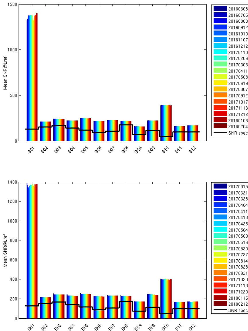
Figure 6: Evolution of the SNR performance of S2A since 08/06/2016 (top) and S2B since 15/03/2017 (bottom)
