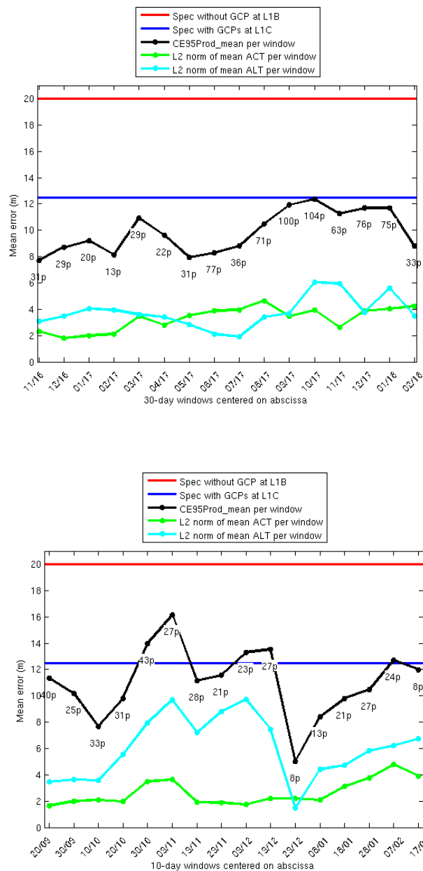
Figure 1: Geolocation performance for S2A (top) and S2B (bottom). The performance is computed over a sliding window of 30 (respectively 10) days for S2A (resp. S2B). (ACT= across track, ALT = along track)
