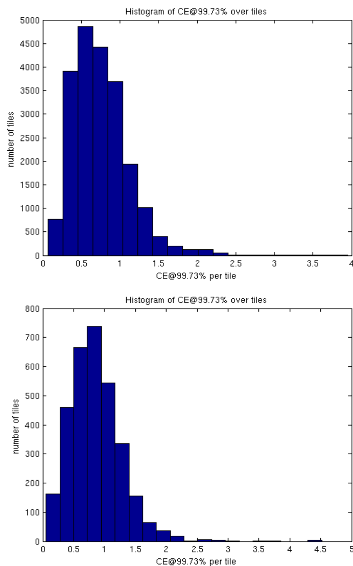
Figure 2: Histogram of the multi-temporal performance for S2A (top) and S2B (bottom, different scale). The 3 m requirement will be applicable only after activation of the geometrical refinement.
