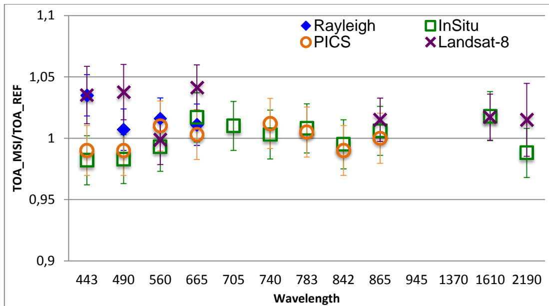
Figure 4: Comparison of radiometric accuracy for all spectral bands (except B09 and B10): ratio of S2A measurement on reference. Error bars indicate the method uncertainty.
