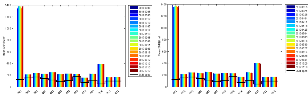
Figure 6: Evolution of the SNR performance of S2A since 08/06/2016 (left) and S2B since 15/03/2017 (right)
