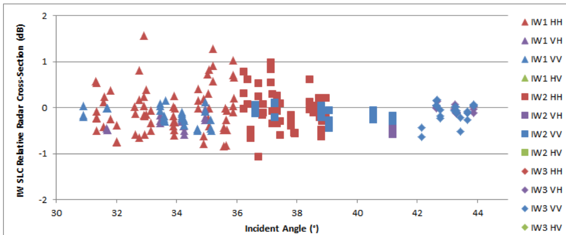
Figure 5 IW Relative Radar Cross-Section
