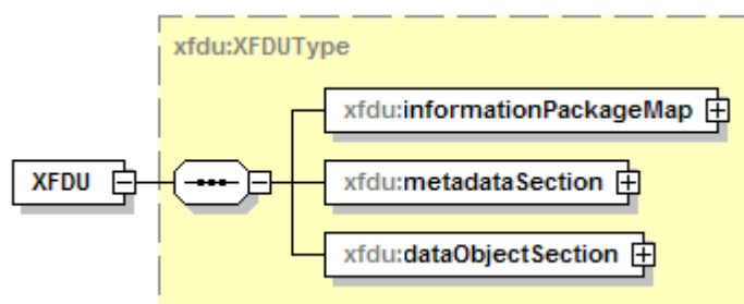
Figure 6-1 Sentinel-1 Manifest File Structure
