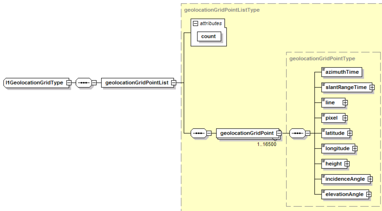
Figure 6-20 L1 Geo-location Grid ADJR
