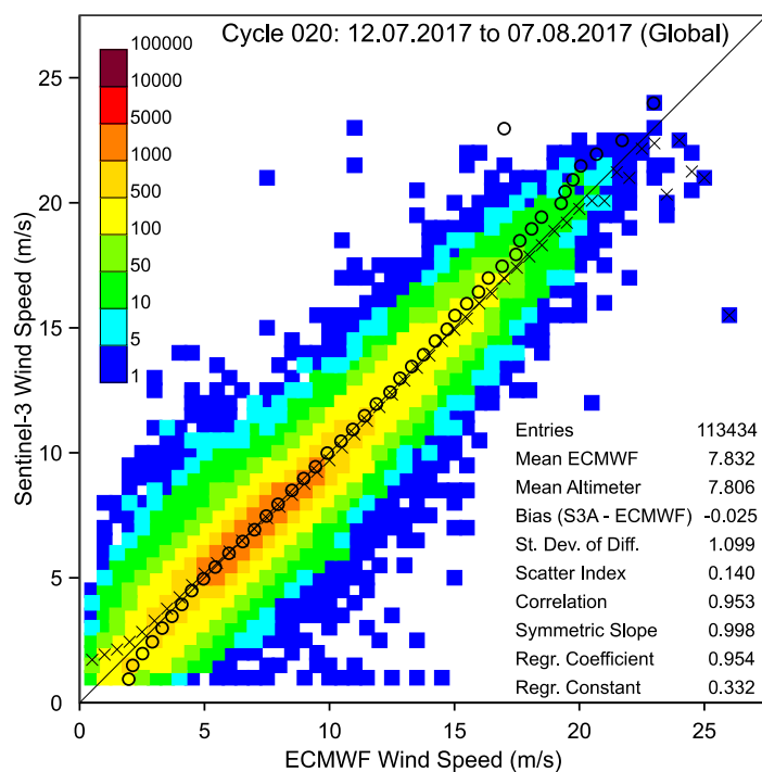
Figure 4: Global comparison between Sentinel-3A SRAL and ECMWF model analysis surface wind speed values over the period of Cycle 020. The number of collocations in each 0.5 m/s x 0.5 m/s 2D bin is color-coded as in the legend. The "x" symbols are the means of the bins for given x-axis values (model) while the "o" symbols are the means for given y-axis values (Sentinel-3).
