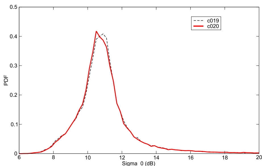
Figure 1: Sentinel-3A SRAL ocean Ku-band backscatter histogram (PDF) over the whole globe and for the period of Cycle 020. For comparison, the same plot from the previous cycle is shown as dashed black line.
