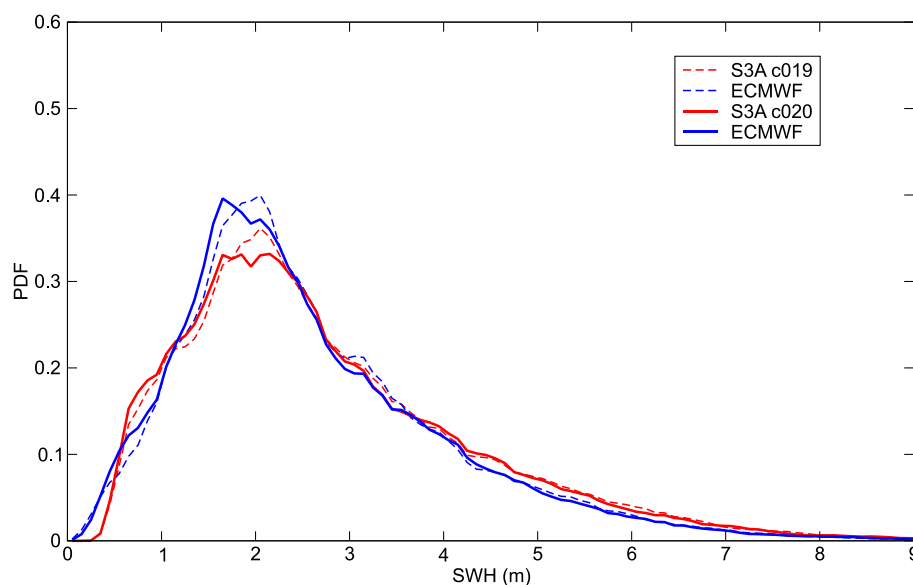
Figure 13: Sentinel-3A SRAL SWH PDF over the whole global ocean and for the period of Cycle 020. The corresponding ECMWF (collocated with Sentinel-3) PDF is also shown for comparison. The corresponding PDF's from the previous cycle are also shown as thin dashed lines.
