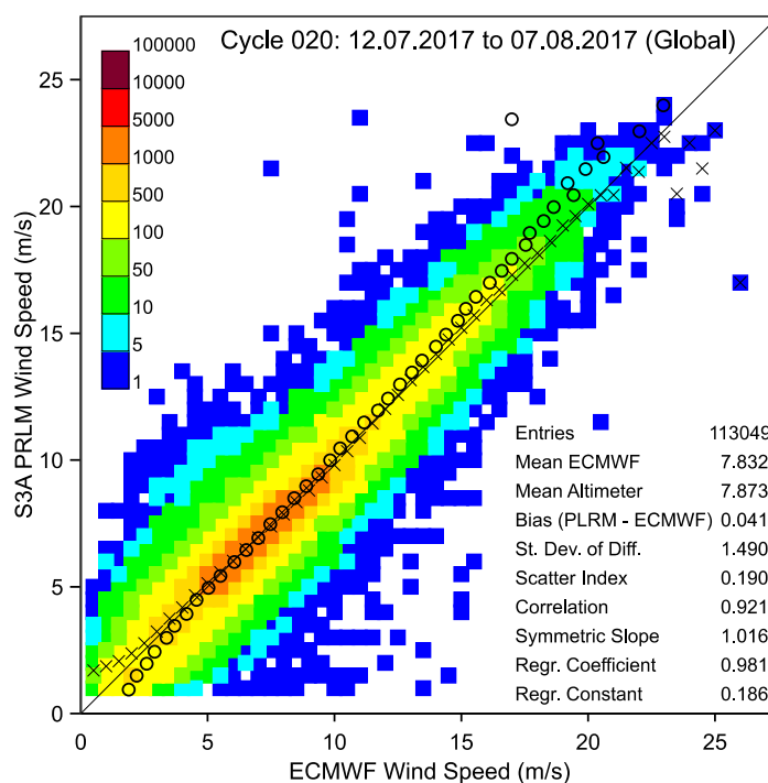
Figure 10: Global comparison between Sentinel-3A PLRM and ECMWF model analysis wind speed values over the period of Cycle 020. Refer to Figure 4 for the meaning of the “x” and “o” symbols as well as the colour coding.
