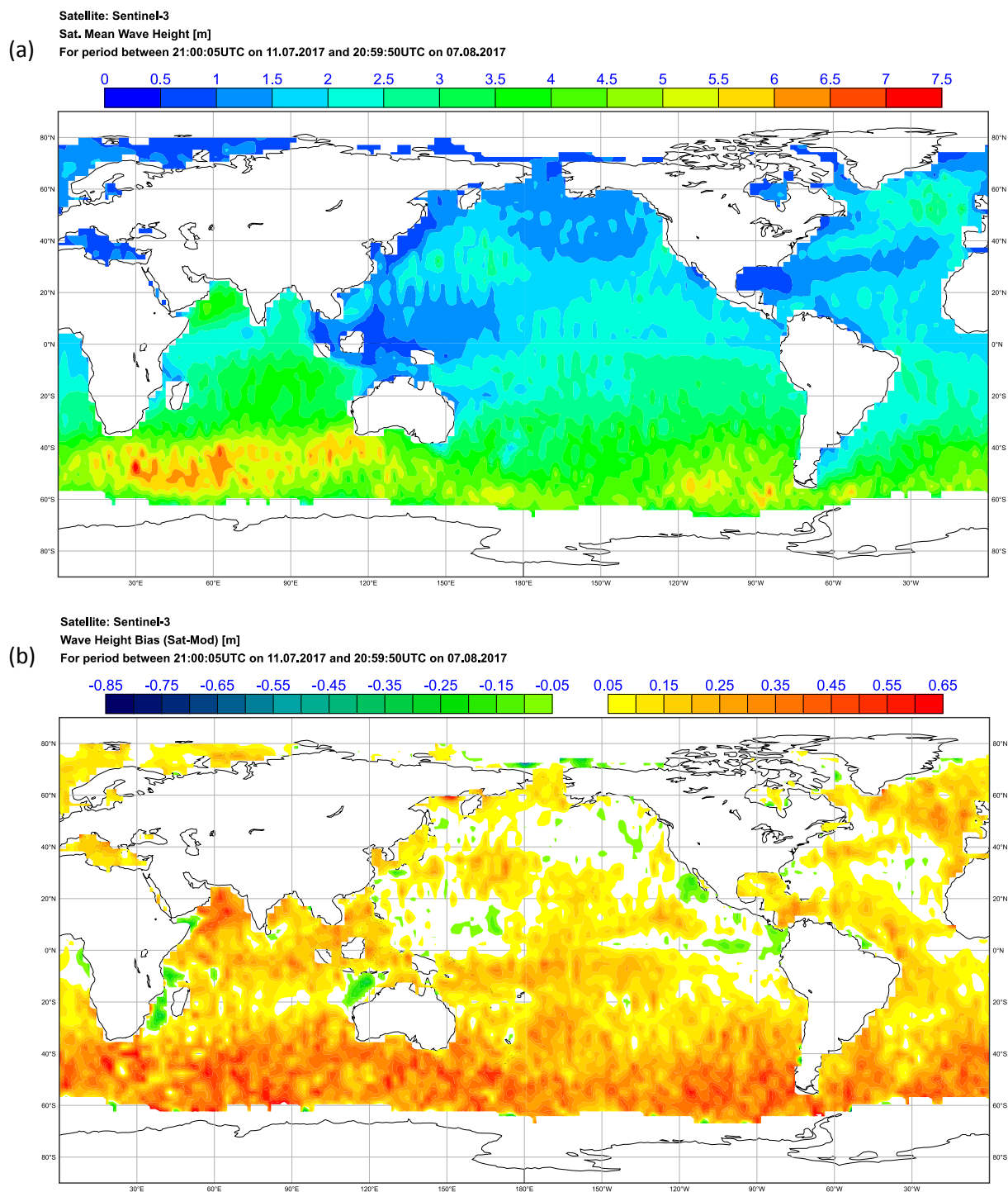
Figure 18: Geographical distribution of mean Sentinel-3 SWH (a) as well as the bias (b); the SDD (c) and the SI (d) between Sentinel-3 and ECMWF model FG during Cycle 020. Bias is defined as altimeter – model.
