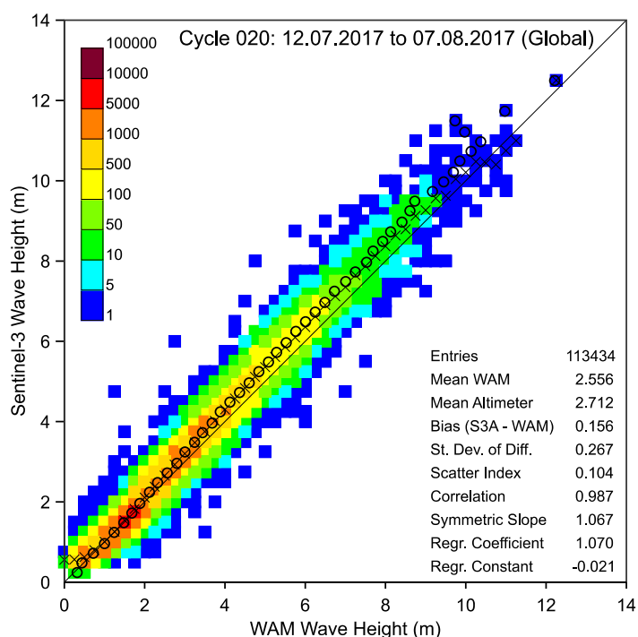
Figure 14: Global comparison between Sentinel-3A and ECMWF model first-guess significant wave height values over the period of Cycle 020. The number of collocations in each 0.25 m x 0.25 m 2D bin is coded as in the legend. Refer to Figure 4 for the meaning of the “x” and “o” symbols.
