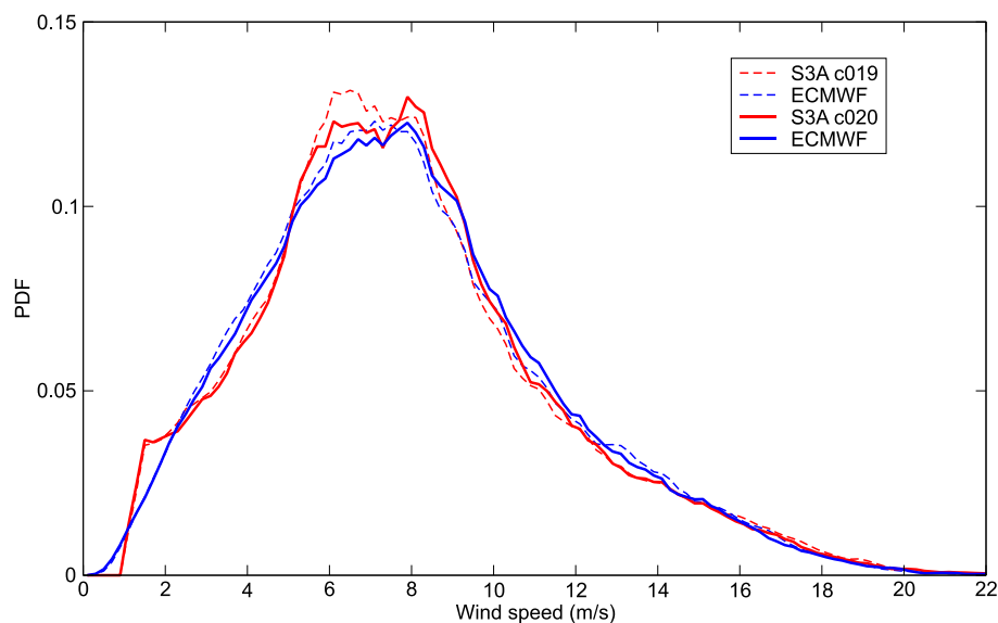
Figure 3: Sentinel-3A SRAL surface wind speed PDF over the whole global ocean and for the period of Cycle 020. The corresponding ECMWF (collocated with Sentinel-3) PDF is also shown for comparison. The corresponding PDF's from the previous cycle are also shown as thin dashed lines.
