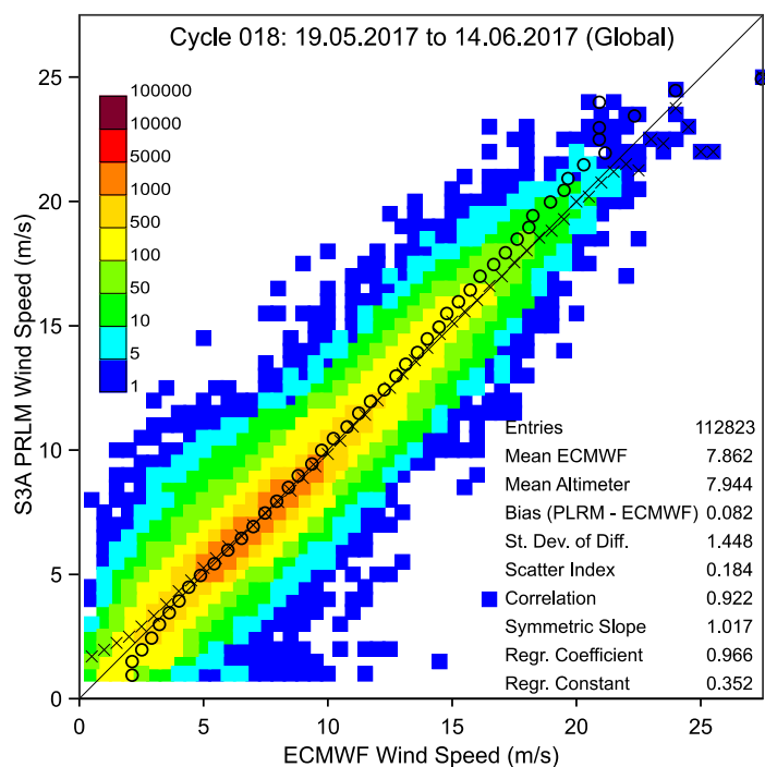
Figure 10: Global comparison between Sentinel-3A PLRM and ECMWF model analysis wind speed values over the period of Cycle 018. Refer to Figure 4 for the meaning of the "x" and "o" symbols as well as the colour coding.
