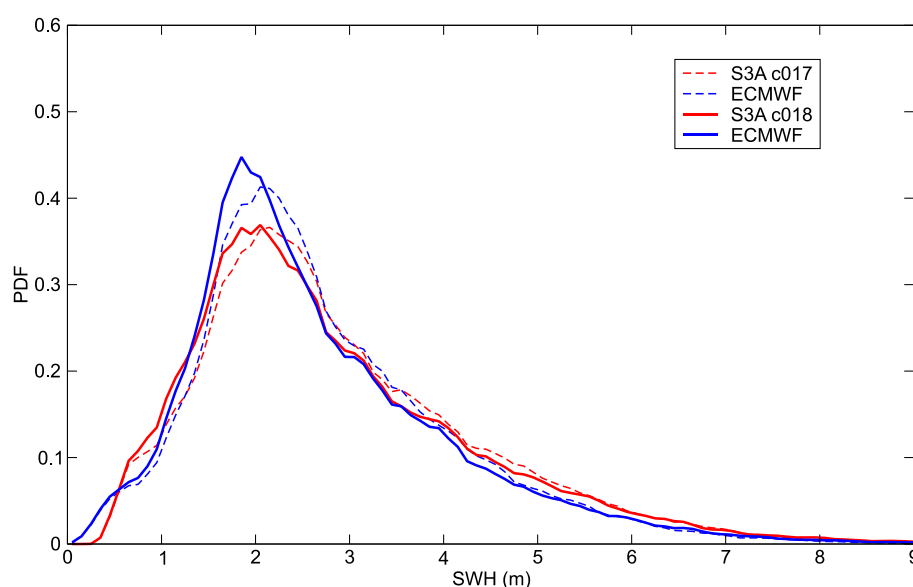
Figure 13: Sentinel-3A SRAL SWH PDF over the whole global ocean and for the period of Cycle 018. The corresponding ECMWF (collocated with Sentinel-3) PDF is also shown for comparison. The corresponding PDF's from the previous cycle are also shown as thin dashed lines.
