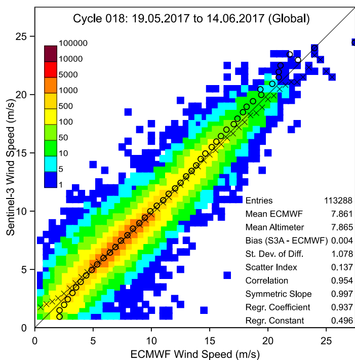
Figure 4: Global comparison between Sentinel-3A SRAL and ECMWF model analysis surface wind speed values over the period of Cycle 018. The number of collocations in each 0.5 m/s x 0.5 m/s 2D bin is color-coded as in the legend. The "x" symbols are the means of the bins for given x-axis values (model) while the "o" symbols are the means for given y-axis values (Sentinel-3).
