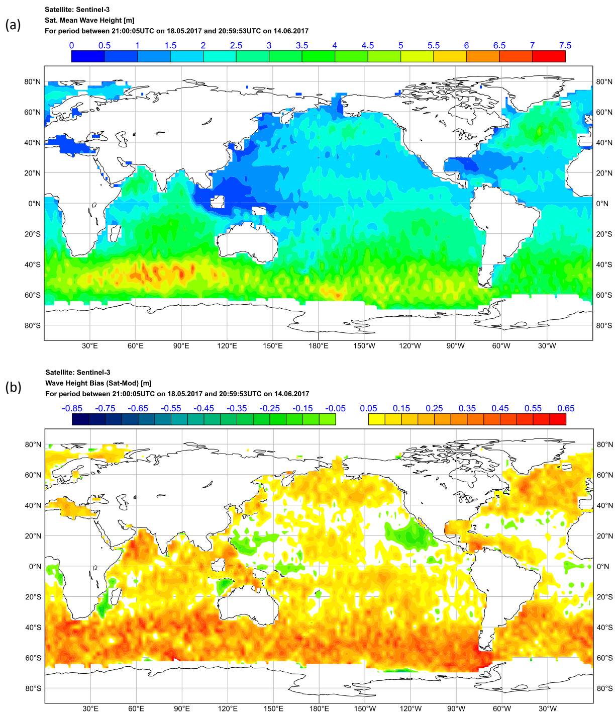
Figure 18: Geographical distribution of mean Sentinel-3 SWH (a) as well as the bias (b); the SDD (c) and the SI (d) between Sentinel-3 and ECMWF model FG during Cycle 018. Bias is defined as altimeter – model.
