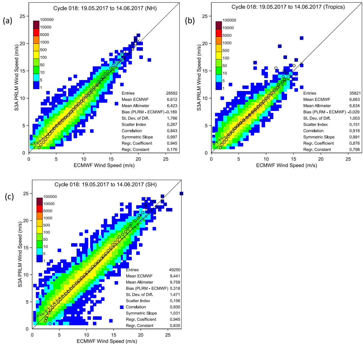
Figure 11: Same as Figure 10 but for Northern Hemisphere (latitudes to the north of 20°N), Tropics (latitudes between 20°S and 20°N) and Southern Hemisphere (latitudes to the south of 20°S), respectively.
