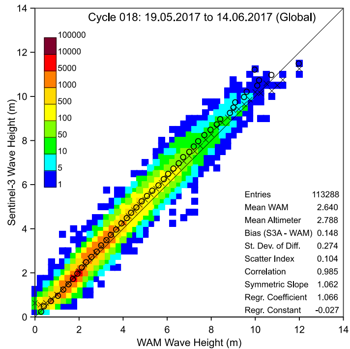
Figure 14: Global comparison between Sentinel-3A and ECMWF model first-guess significant wave height values over the period of Cycle 018. The number of collocations in each 0.25 m x 0.25 m 2D bin is coded as in the legend. Refer to Figure 4 for the meaning of the “x” and “o” symbols.
