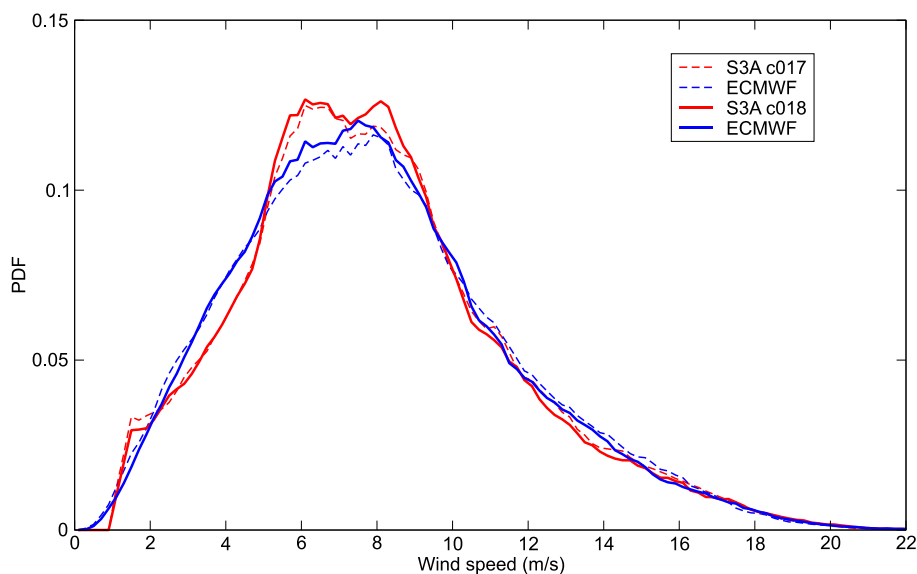
Figure 3: Sentinel-3A SRAL surface wind speed PDF over the whole global ocean and for the period of Cycle 018. The corresponding ECMWF (collocated with Sentinel-3) PDF is also shown for comparison. The corresponding PDF's from the previous cycle are also shown as thin dashed lines.
