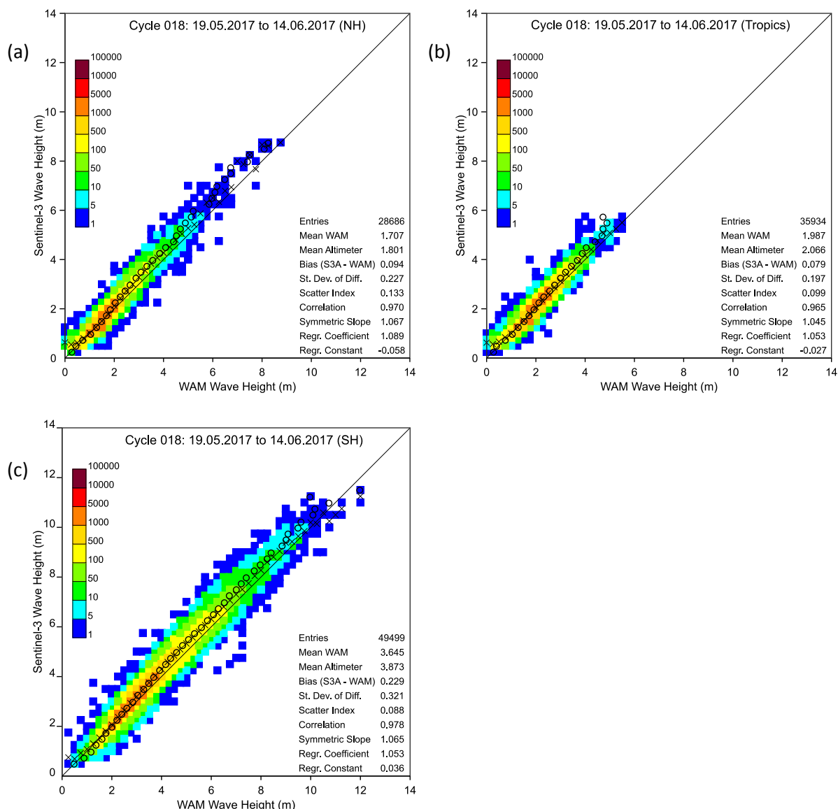
Figure 15: Same as Figure 14 but for Northern Hemisphere (latitudes to the north of 20° N), Tropics (latitudes between 20°S and 20°N) and Southern Hemisphere (latitudes to the south of 20°S), respectively.
