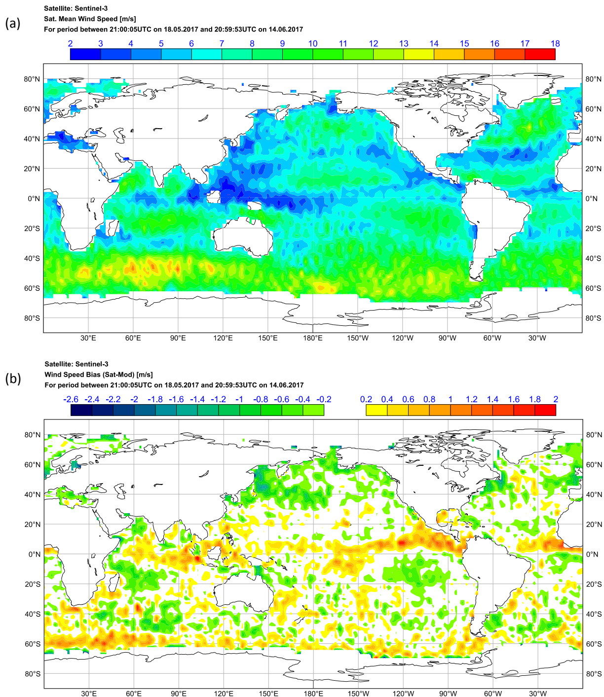
Figure 8: Geographical distribution of mean Sentinel-3 wind speed (a) as well as the bias (b); the SDD (c) and the SI (d) between Sentinel-3 and ECMWF model AN during Cycle 018. Bias is defined as altimeter – model.
