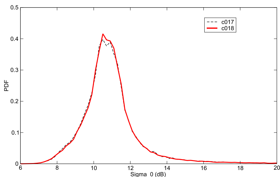
Figure 1: Sentinel-3A SRAL ocean Ku-band backscatter histogram (PDF) over the whole globe and for the period of Cycle 018. For comparison, the same plot from the previous cycle is shown as dashed black line.
