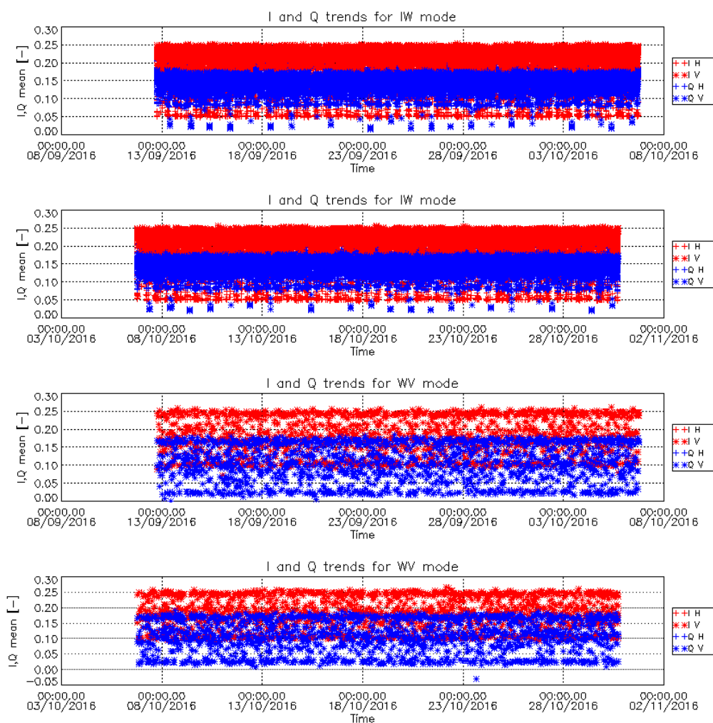
Figure 2 I&Q Channels
