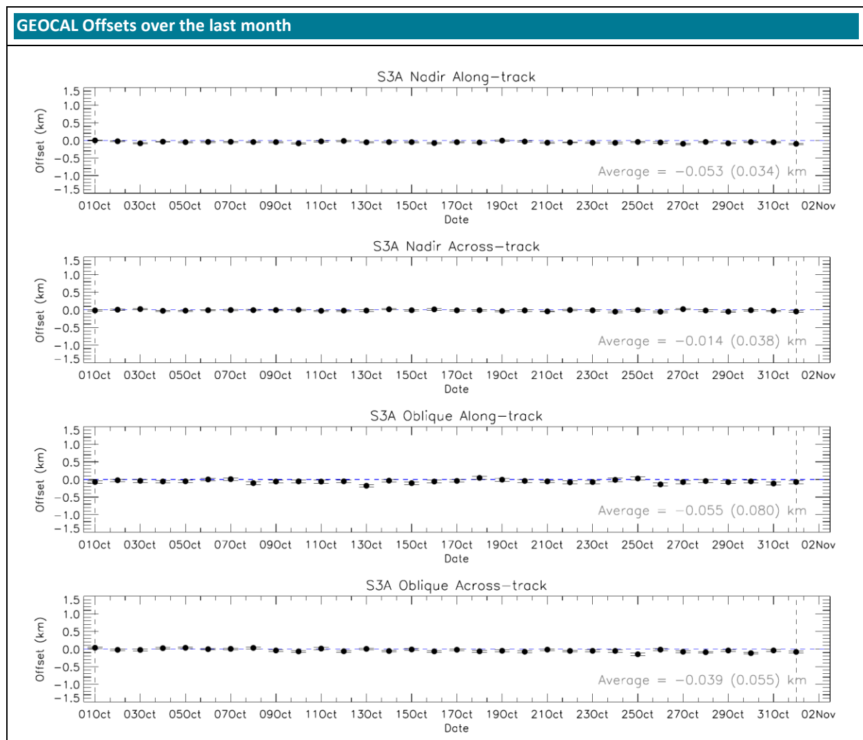
Figure 26: SLSTR-A daily offset results in km from the GeoCal Tool analysis for Nadir along- and across-track (top two plots) and Oblique along- and across-track (bottom two plots) for October 2023. The error bars show the standard deviation.
