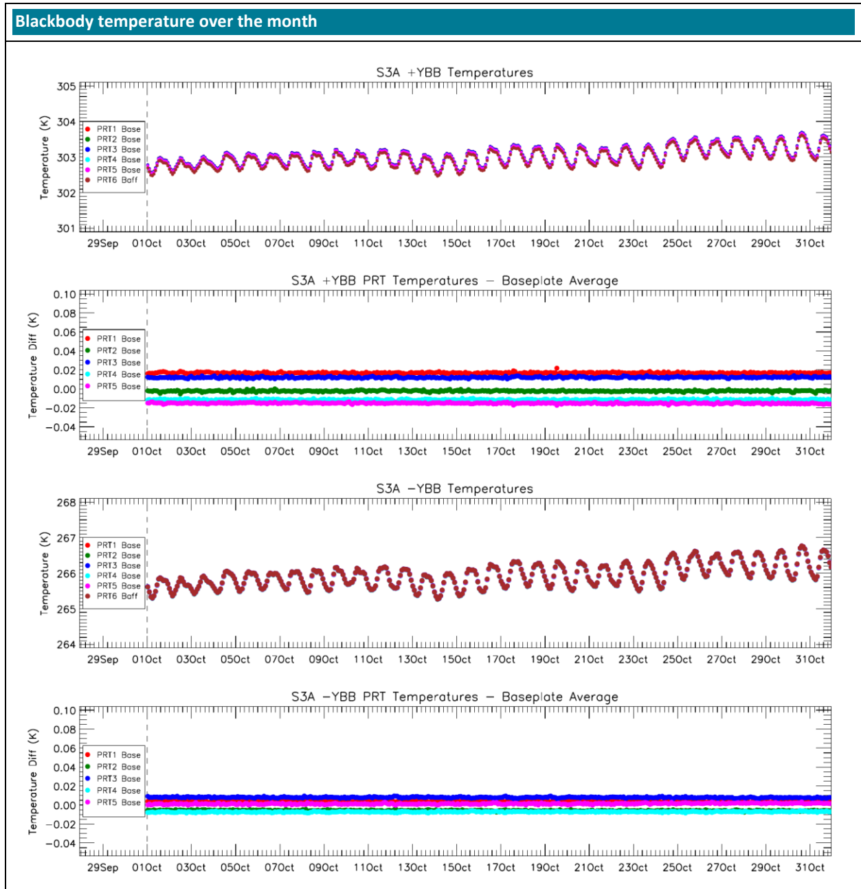
Figure 8: SLSTR-A blackbody temperature and baseplate gradient trends during October 2023 measured by different sensors at various positions in the BB and Baseplate. Each dot represents the average temperature in one orbit.
