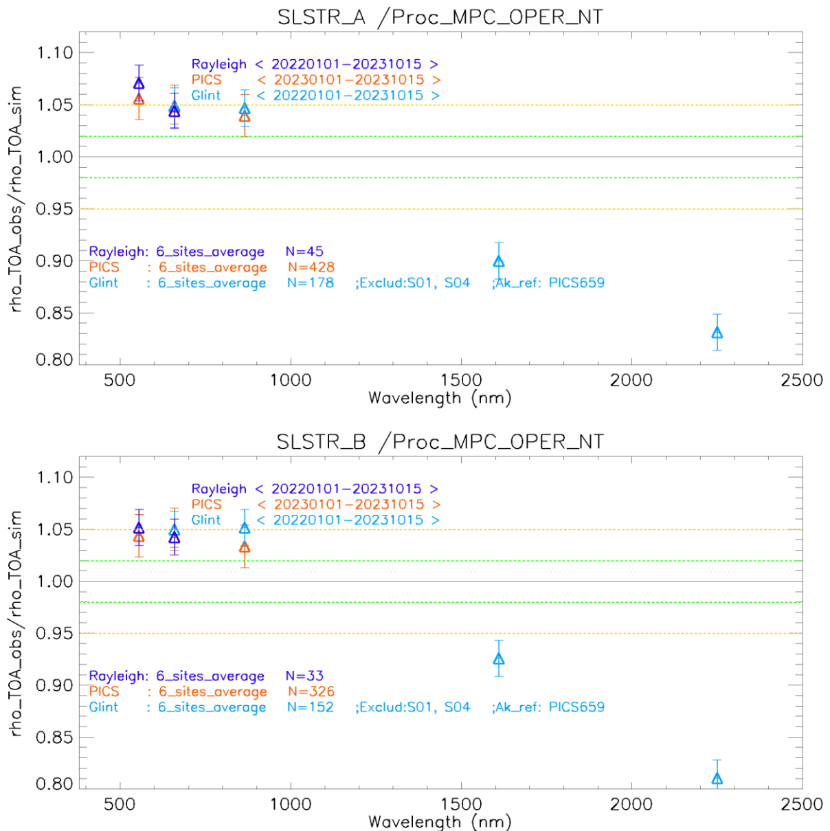
Figure 24: The estimated gain values for SLSTR-A and SLSTR-B (Nadir view) from Glint and Rayleigh methods over the period Jan 2022—mid-October 2023 and PICS method over the period Jan 2023—mid-October 2023 as a function of wavelength. We use the gain value of S02 from Desert-PICS method as reference gain for Glint method. Dashed-green and orange lines indicate the 2% and 5% respectively. Error bars indicate the method uncertainties.
