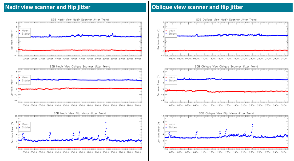
Figure 6: SLSTR-B scanner and flip jitter for October 2023, showing mean and stddev difference from expected position per orbit (red and blue respectively) for the nadir view (left) and oblique view (right). The plots show the nadir scanner (top), oblique scanner (middle) and flip mirror (bottom).
