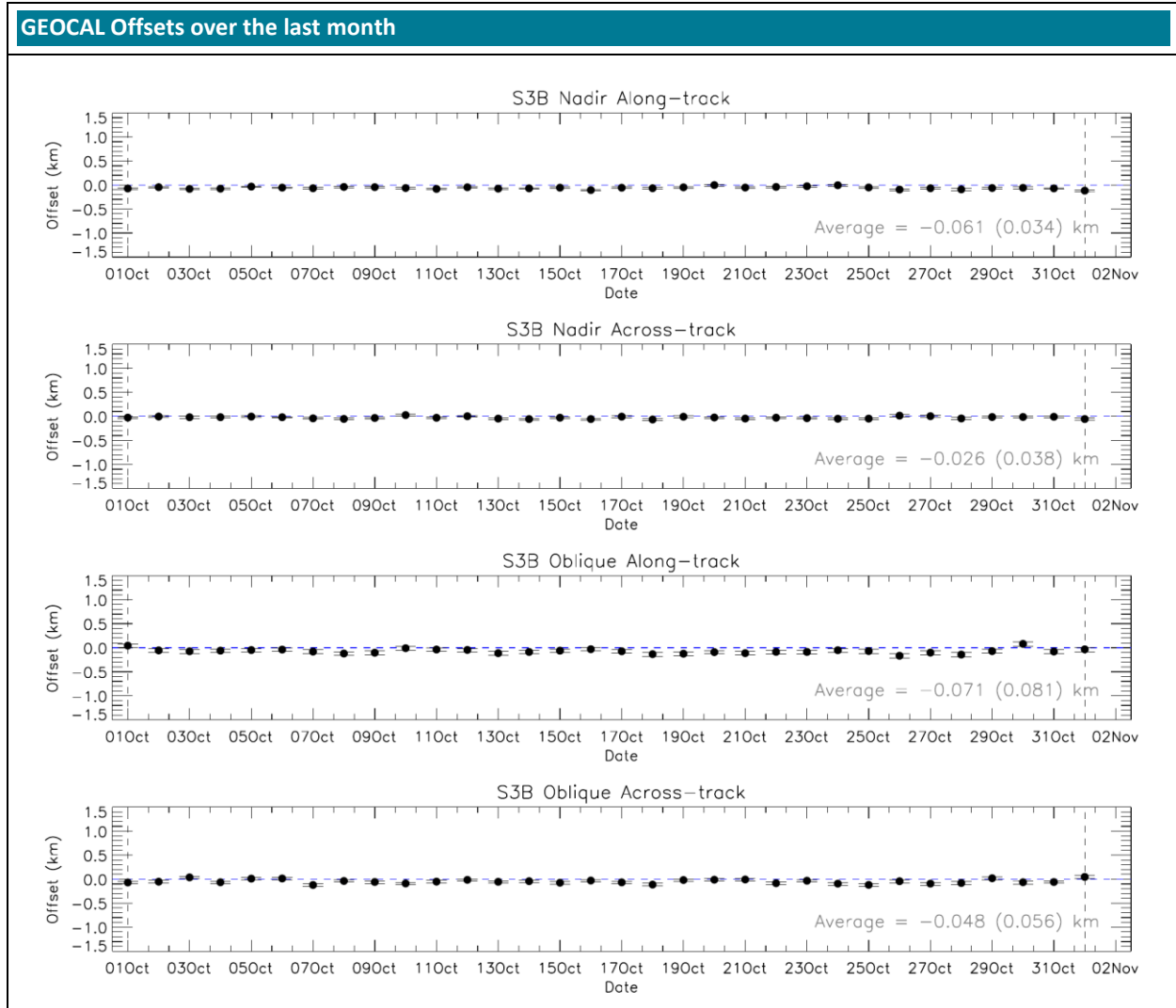
Figure 27: SLSTR-B daily offset results in km from the GeoCal Tool analysis for Nadir along- and across-track (top two plots) and Oblique along- and across-track (bottom two plots) for October 2023. The error bars show the standard deviation.
