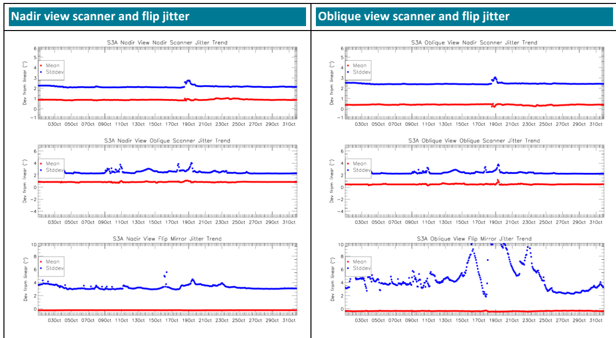
Figure 5: SLSTR-A scanner and flip jitter for October 2023, showing mean and stddev from expected position per orbit (red and blue respectively) for the nadir view (left) and oblique view (right). The plots show the nadir scanner (top), oblique scanner (middle) and flip mirror (bottom).
