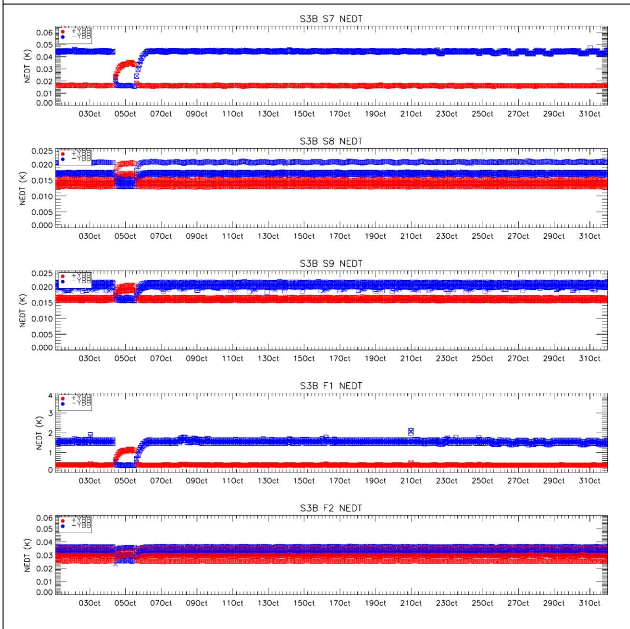
Figure 15: SLSTR-B NEDT trend for the thermal channels in October 2023. Blue points were calculated from the cold blackbody signal and red points from the hot blackbody. The square symbols show results calculated from the nadir view and crosses show results from the oblique view. Results are plotted for all detectors and integrators, which is why there are several different levels within the same colour points (particularly for S8 and F2). A blackbody cross over test was performed this month, which can be observed in the data near the 4-5 th .
