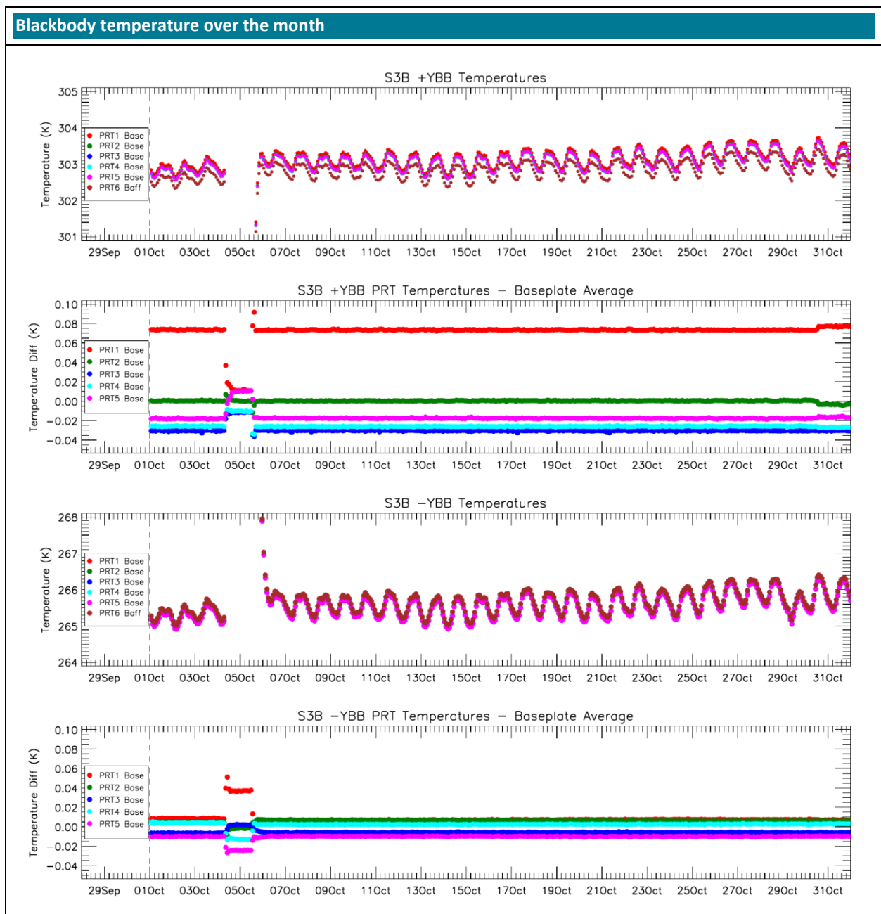
Figure 9: SLSTR-B blackbody temperature and baseplate gradient trends during October 2023 measured by different sensors at various positions in the BB and Baseplate. Each dot represents the average temperature in one orbit.
