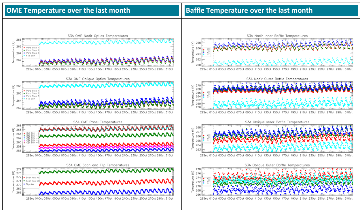
Figure 1: OME temperature trends for SLSTR-A (left) and Baffle temperature trends (right) during October 2023. The OME plot shows the three paraboloid stops and flip baffle (top two plots) and optical bench at different positions (third plots), and scanner and flip assembly (bottom plots). The Baffle plot shows the temperature at different positions on the inner and outer baffles. Each dot represents the average temperature in one orbit.
