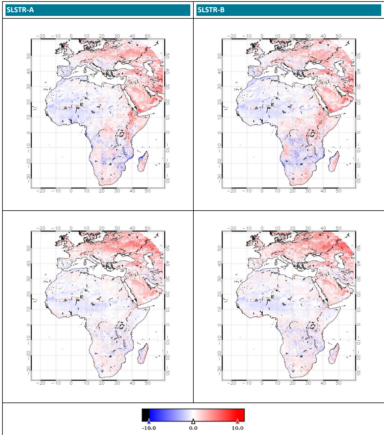
Figure 29: Intercomparison of the SL_2_LST product with respect to the operational LSA SAF SEVIRI LST product for December 2022 for SLSTR-A (left) and SLSTR-B (right). Daytime composites are in the top row and Night-time composites are in the bottom row.
