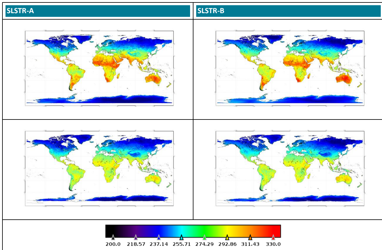
Figure 30: Monthly composites at 0.05^\circ of LST for December 2022 for SLSTR-A (left) and SLSTR-B (right). Daytime composites are in the top row and Night-time composites are in the bottom row.
