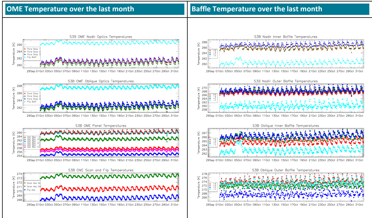
Figure 2: SLSTR-B OME temperature trends (left) and Baffle temperature trends (right) during October 2023. The OME plot shows the three paraboloid stops and flip baffle (top two plots) and optical bench at different positions (third plots), and scanner and flip assembly (bottom plots). The Baffle plot shows the temperature at different positions on the inner and outer baffles. Each dot represents the average temperature in one orbit.
