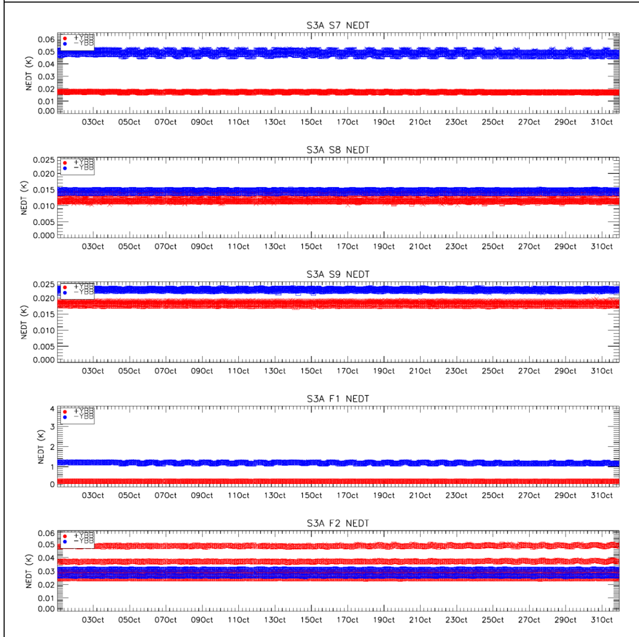
Figure 14: SLSTR-A NEDT trend for the thermal channels in October 2023. Blue points were calculated from the cold blackbody signal and red points from the hot blackbody. The square symbols show results calculated from the nadir view and crosses show results from the oblique view. Results are plotted for all detectors and integrators, which is why there are several different levels within the same colour points (particularly for S8 and F2).
