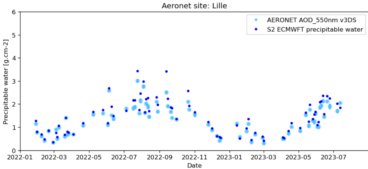
Figure 10: Total Water Column [g.cm-2]; AERONET data (light blue) and S2 ECMWFT data (blue) Lille: Tile 31UES Sentinel-2 products between 25/01/2022 and 21/08/2023
