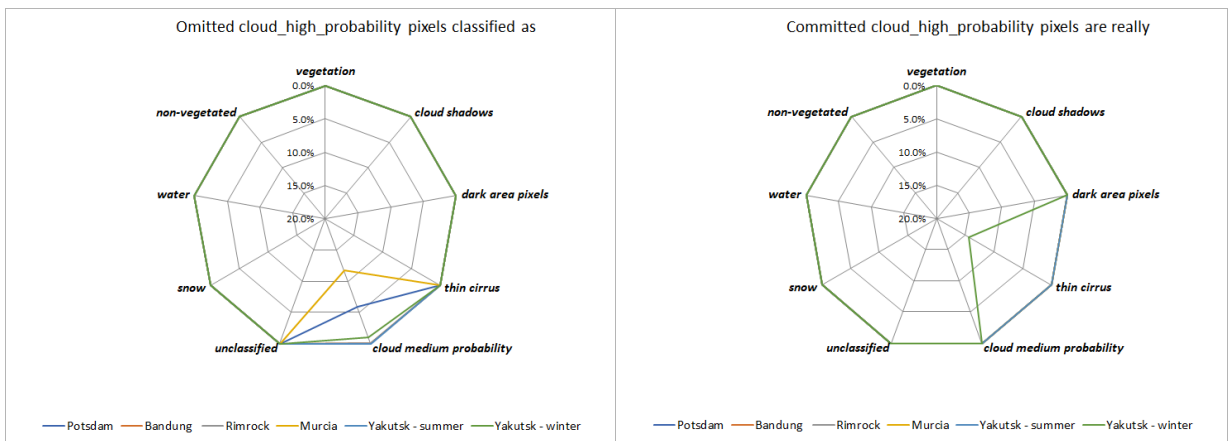
Figure 7: Spider plots of the omission and commission errors of cloud high probability pixels
