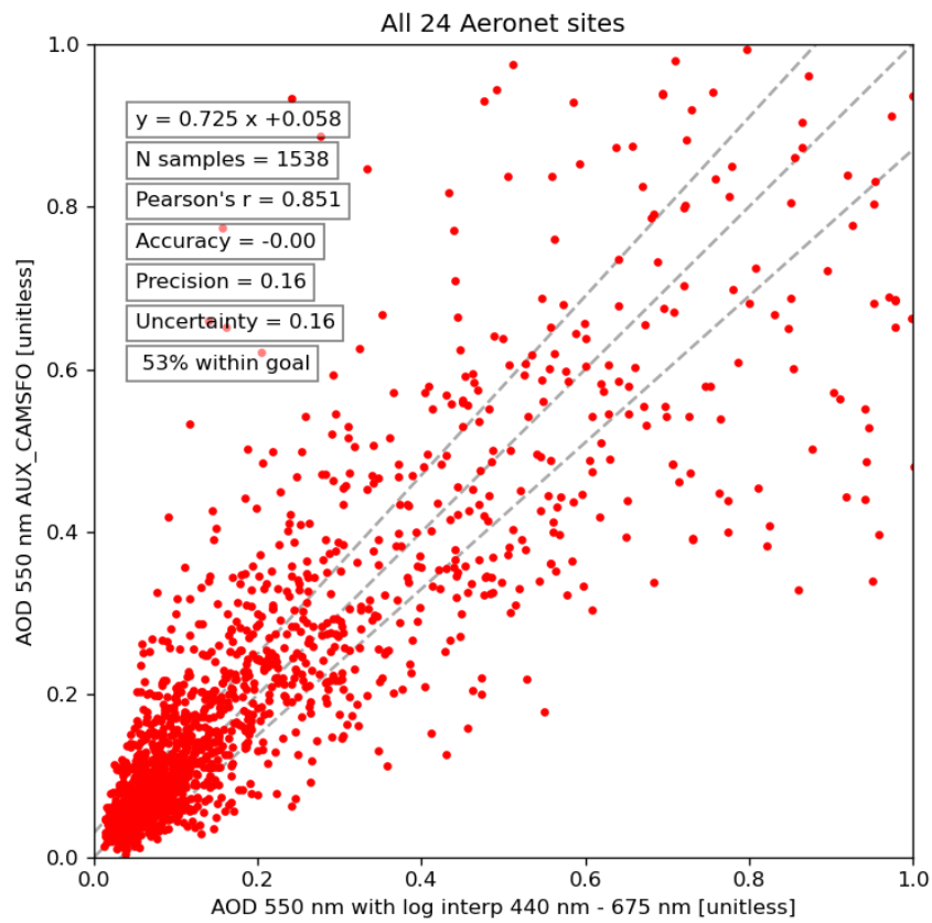
Figure 9: Aerosol Optical Depth at 550 nm; scatter plot S2 CAMS data vs AERONET data 24 test sites: Sentinel-2 products between 25/01/2022 and 25/06/2023
