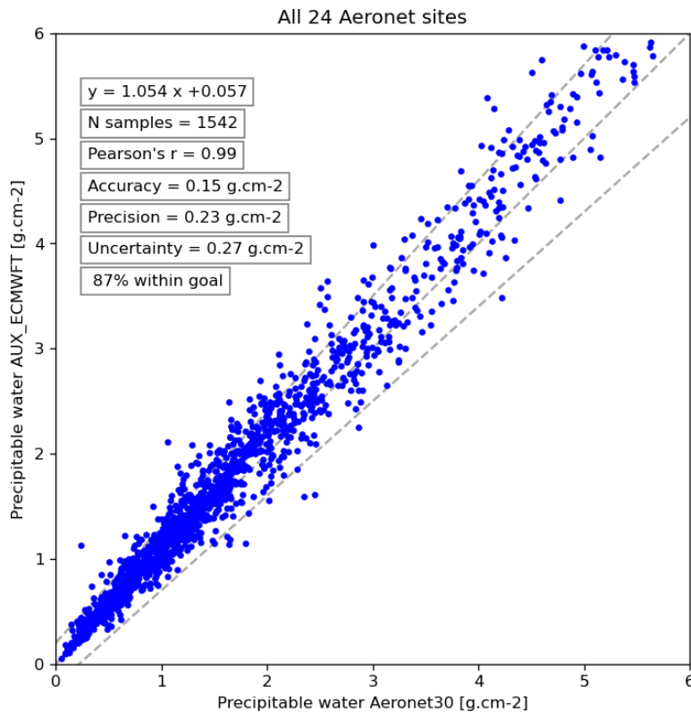
Figure 11: Total Water Column [g.cm-2]; scatter plot S2 ECMWFT data vs AERONET data 24 test sites: Sentinel-2 products between 25/01/2022 and 21/08/2023
