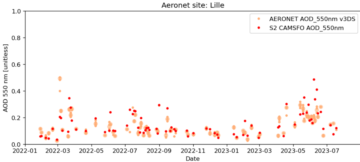
Figure 8: Aerosol Optical Depth at 550 nm; AERONET data (light red) and S2 CAMS data (red) Lille: Tile 31UES Sentinel-2 products between 25/01/2022 and 21/08/2023
