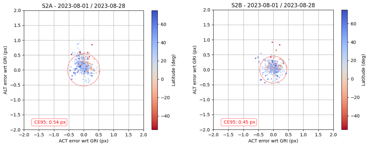
Figure 7: Relative geolocation performance for refined products. Left: S2A, Right: S2B (01.08.2023 – 28.08.2023)
