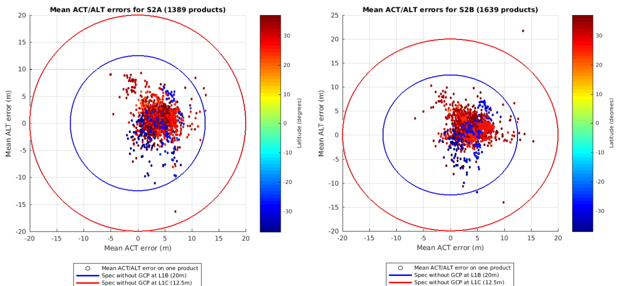
Figure 9: Absolute geolocation performance for refined products. Left: S2A, Right: S2B (01.2022 – 06.2023)
