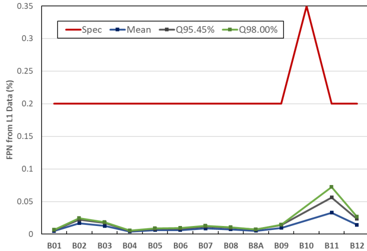
Figure 19 : Fixed Pattern Noise (residual error after equalization) measured on homogeneous natural images for S2A (left) and S2B (right) for July 2023. Blue curve: mean FPN, grey curve: Q95.45%, green curve: Q98.00% and red curve: specified value.
