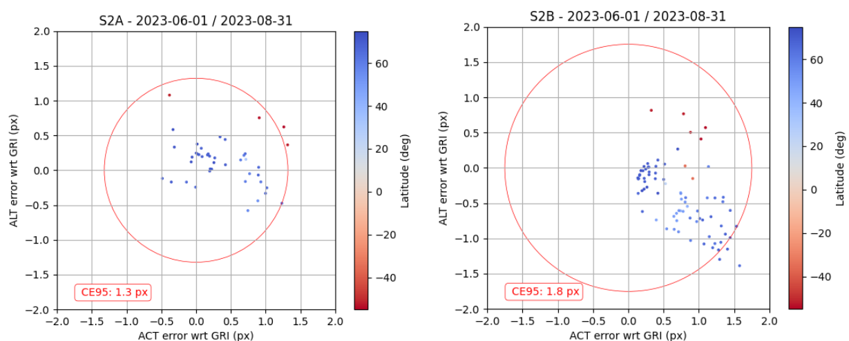
Figure 6: Relative geolocation performance for unrefined products. Left: S2A, Right: S2B (01.06.2023 – 31.06.2023)
