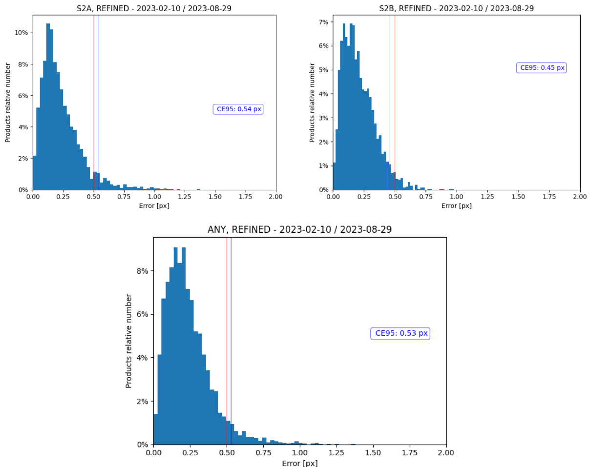
Figure 11: Multi-temporal 2D co-registration errors for refined S2A (left) and S2B pairs (right), and all pairs (bottom) (10.02.2023 to 29.08.2023). The 95.45% performance is around 5 m.
