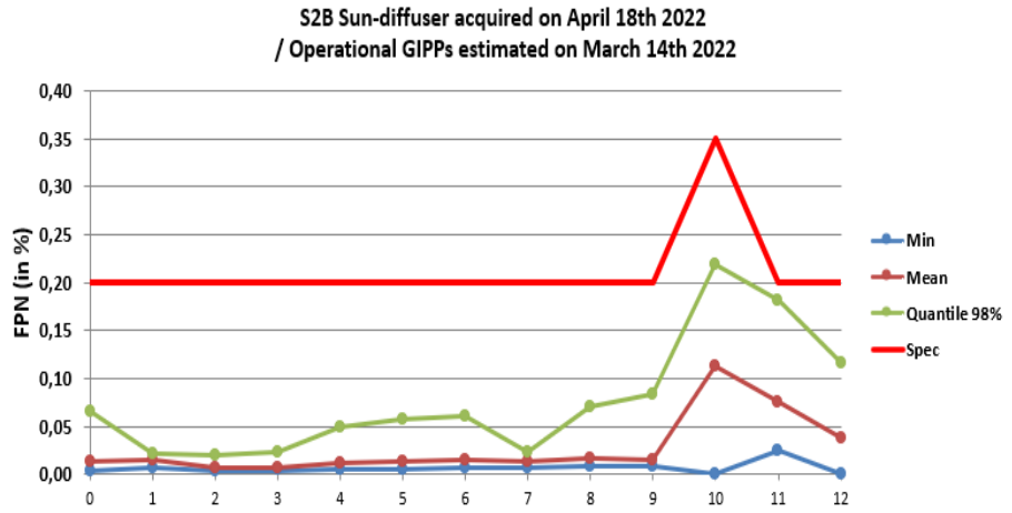
Figure 18: Fixed Pattern Noise (residual error after equalization) measured on diffuser images for S2A (top) and S2B (bottom). Blue curve: min FPN, marron: mean, green: 98 percentile, red: specified value.
