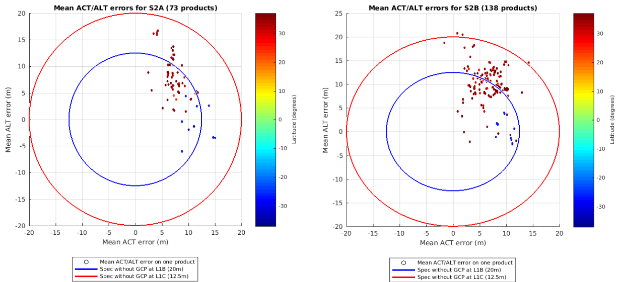
Figure 8: Absolute geolocation performance for unrefined products. Left: S2A, Right: S2B (01.2022 – 04.2023)
