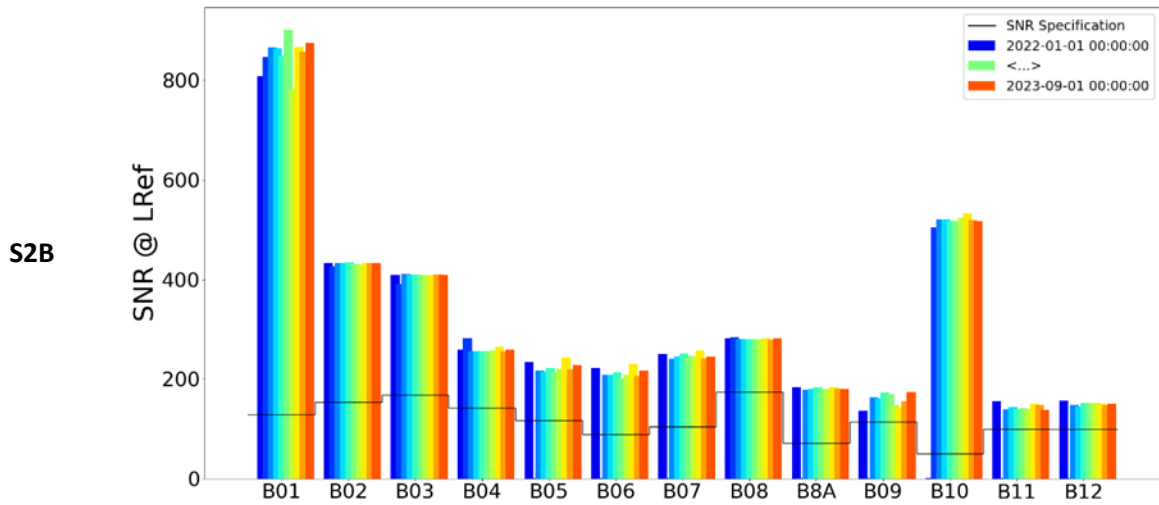
Figure 17 : Evolution of the SNR performances based on homogeneous natural acquisitions for S2A (top) and S2B (bottom) from 01/01/2022 to 01/09/2023
