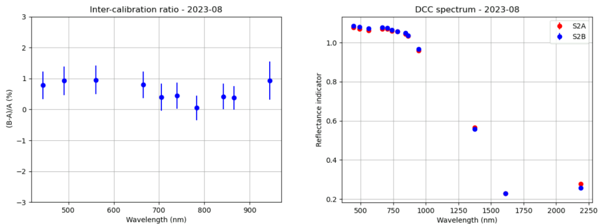
Figure 15 : Inter-calibration ratio between S2A and S2B as a function of the wavelength (left) assessed based on acquisitions from August 2023. Reflectance indicator for all wavebands in the VNIR shows an alignment of S2A compared to S2B following the introduction of the radiometric harmonization factor on 01/2022.
