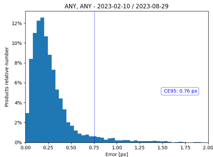
Figure 12: Histogram of the multi-temporal performance for all products (refined and unrefined) (10.02.2023 to 29.08.2023).
