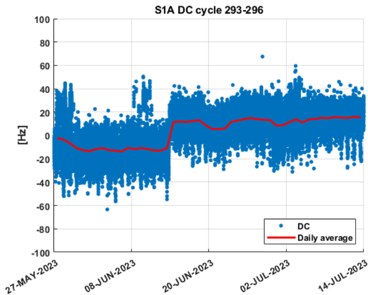
Figure 9 S1-A Doppler Centroid
