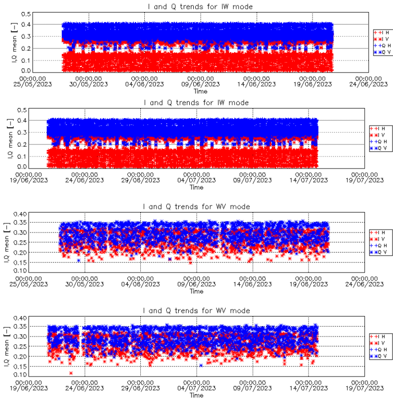
Figure 2 I&Q Channels
