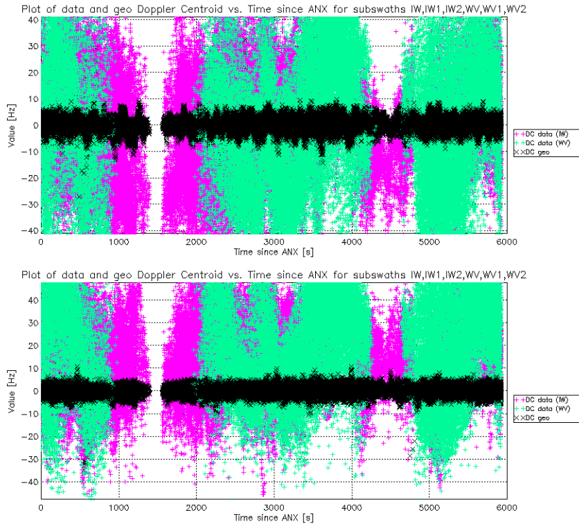
Figure 8 S1-A Doppler Centroid as respect to 1) time (vertical black lines representing the date of manoeuvres) and 2) ANX time (top and bottom respectively cycle 293-294 and cycles 295-296)
