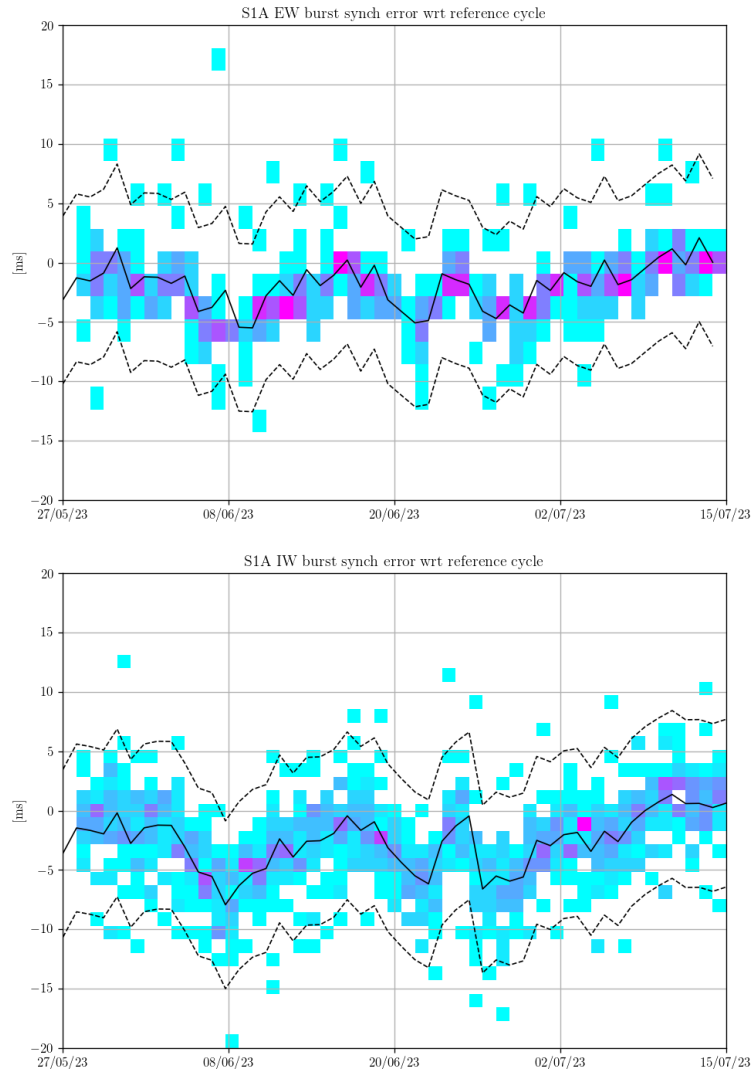
Figure 10: Burst synchronization error for current reporting period. Top image is for EW acquisition mode, bottom is for IW acquisition mode.
