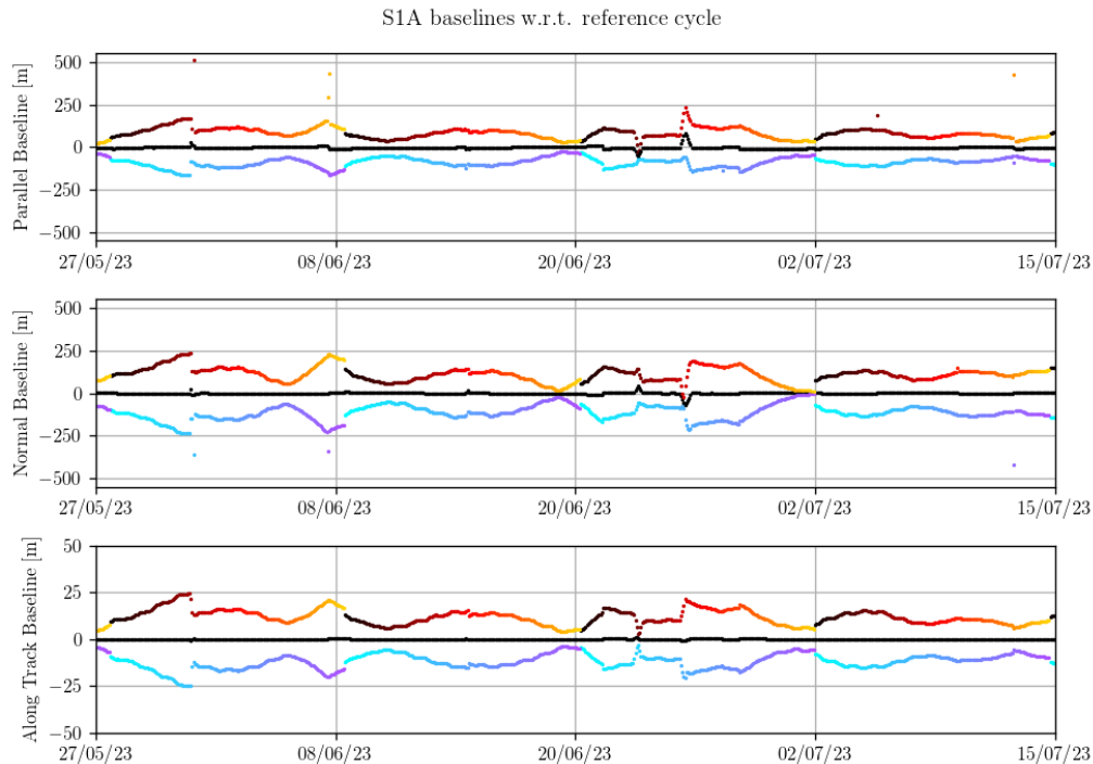
Figure 11: Interferometric baselines for reporting period
